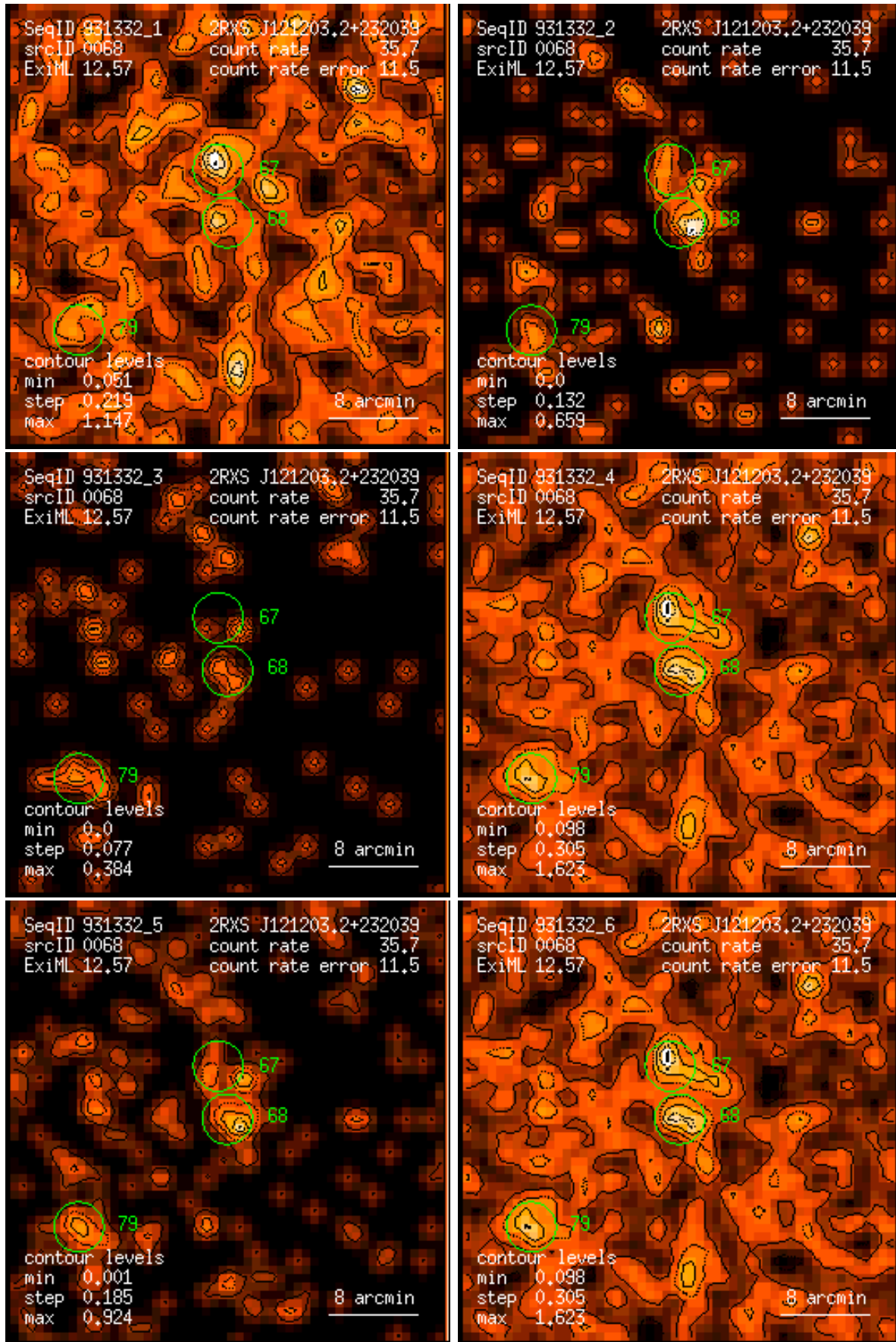
Figure 68: RASS 931332: detection 0068: band rate images, Gaussian filter: (1) PSPC channels 11 – 41, (2) 52 – 90, (3) 91 – 201, (4) 11 – 235, (5) 52 – 201, (6) 11 – 201. Broad band rates in counts/ks. Band rate contour levels in counts/ks/arcmin 2 .
