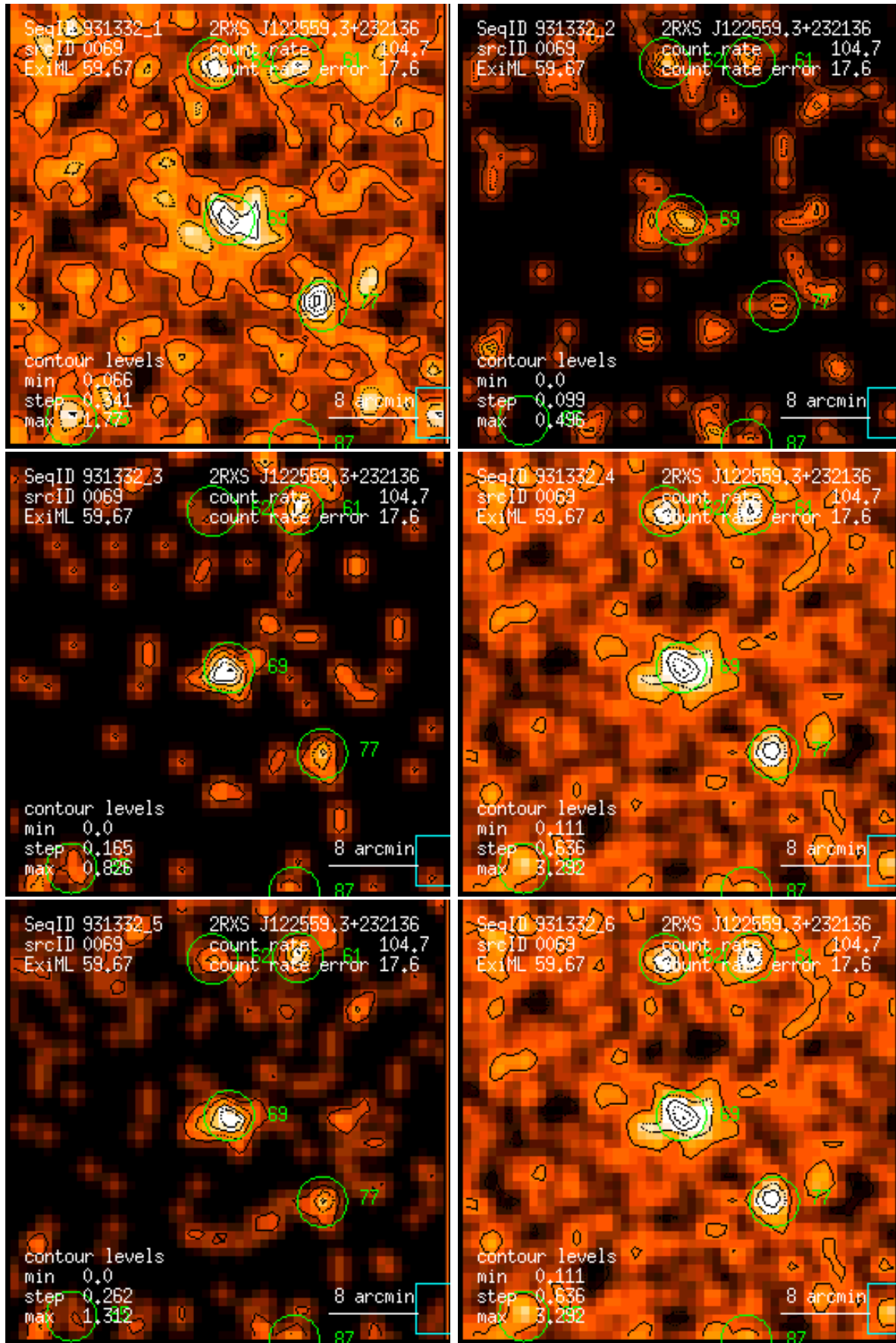
Figure 69: RASS 931332: detection 0069: band rate images, Gaussian filter: (1) PSPC channels 11 – 41, (2) 52 – 90, (3) 91 – 201, (4) 11 – 235, (5) 52 – 201, (6) 11 – 201. Broad band rates in counts/ks. Band rate contour levels in counts/ks/arcmin 2 .
