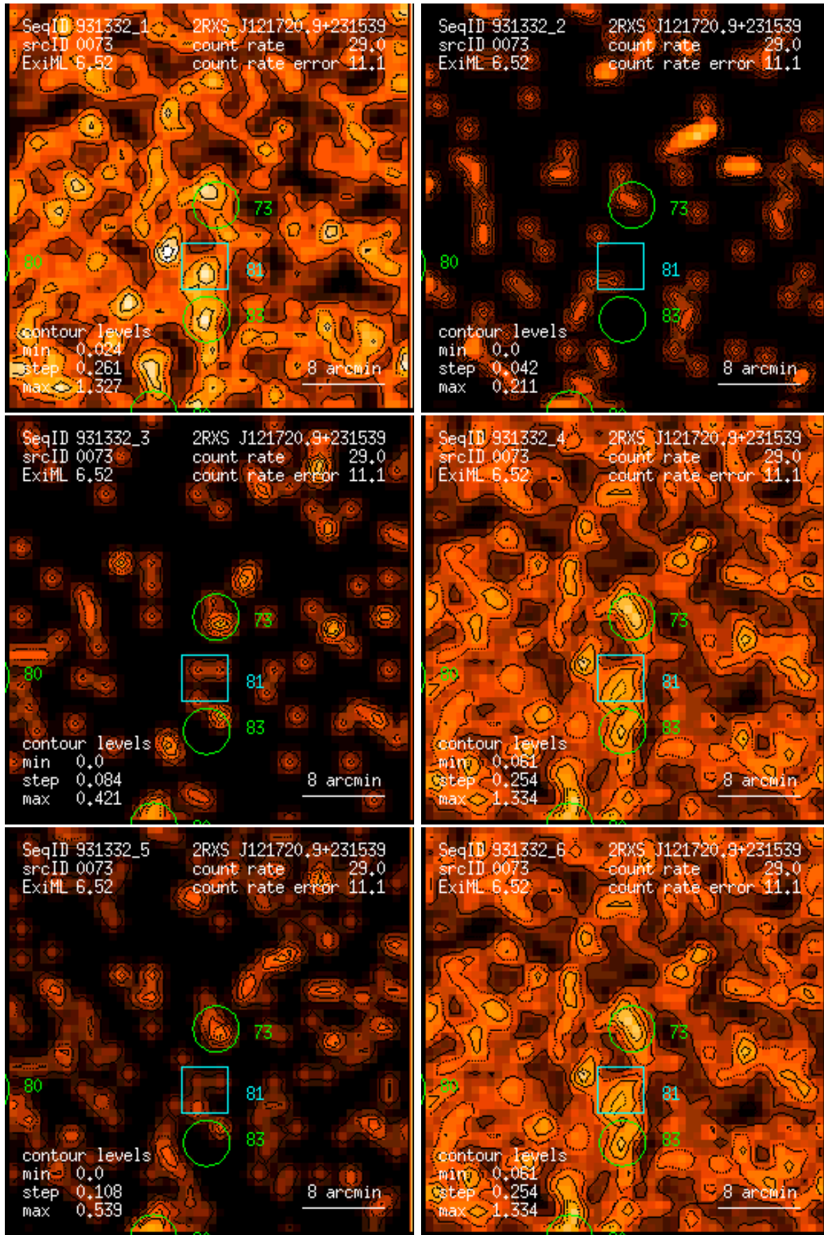
Figure 73: RASS 931332: detection 0073: band rate images, Gaussian filter: (1) PSPC channels 11 – 41, (2) 52 – 90, (3) 91 – 201, (4) 11 – 235, (5) 52 – 201, (6) 11 – 201. Broad band rates in counts/ks. Band rate contour levels in counts/ks/arcmin 2 .
