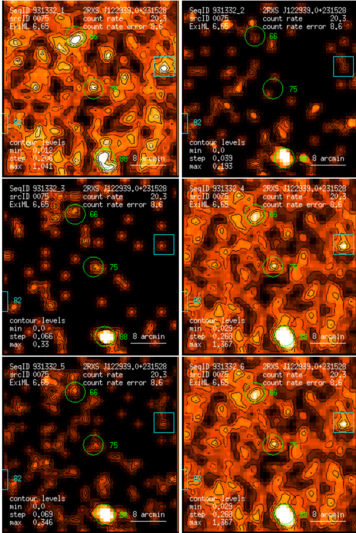
Figure 75: RASS 931332: detection 0075: band rate images, Gaussian filter: (1) PSPC channels 11 – 41, (2) 52 – 90, (3) 91 – 201, (4) 11 – 235, (5) 52 – 201, (6) 11 – 201. Broad band rates in counts/ks. Band rate contour levels in counts/ks/arcmin 2 .
