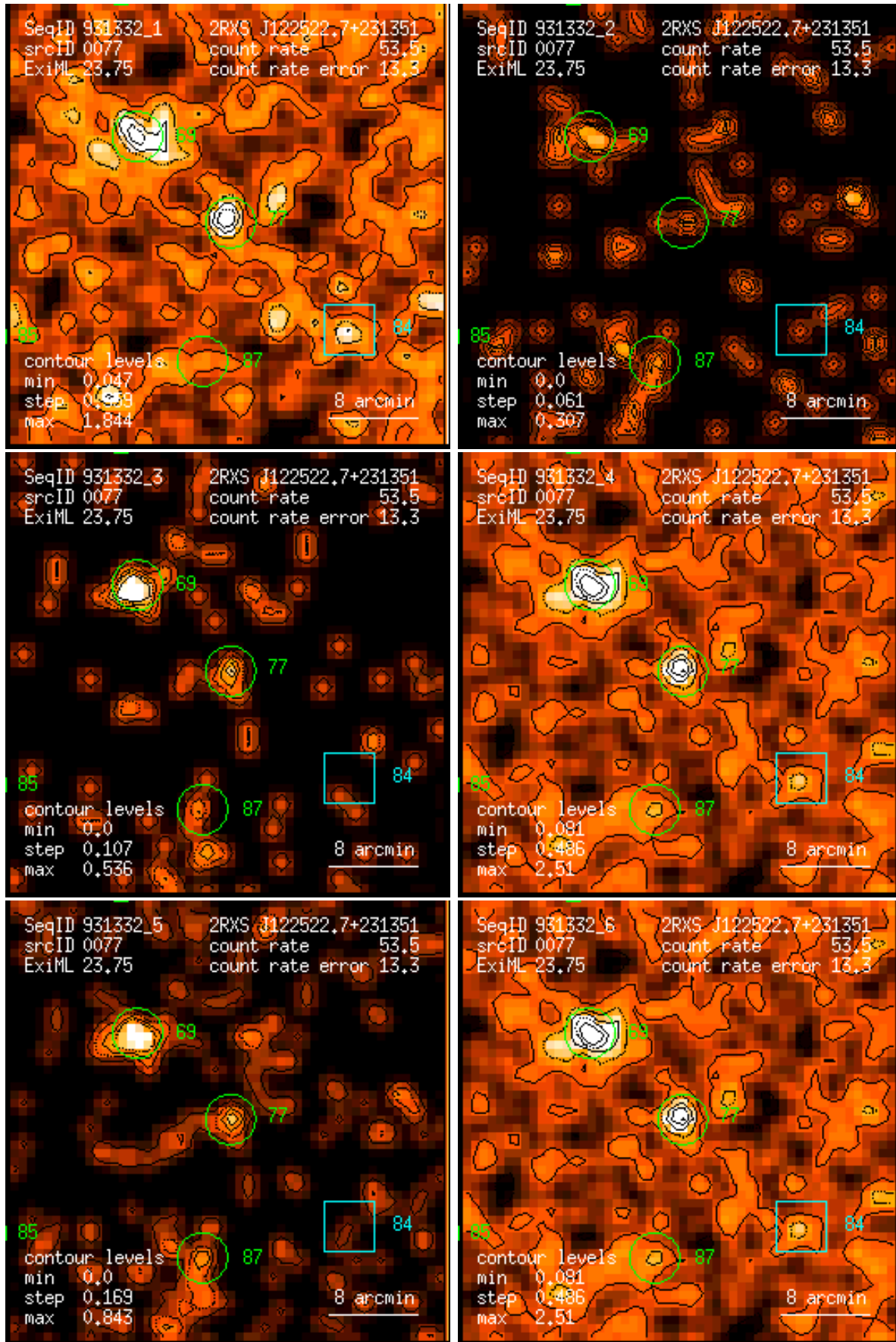
Figure 77: RASS 931332: detection 0077: band rate images, Gaussian filter: (1) PSPC channels 11 – 41, (2) 52 – 90, (3) 91 – 201, (4) 11 – 235, (5) 52 – 201, (6) 11 – 201. Broad band rates in counts/ks. Band rate contour levels in counts/ks/arcmin 2 .
