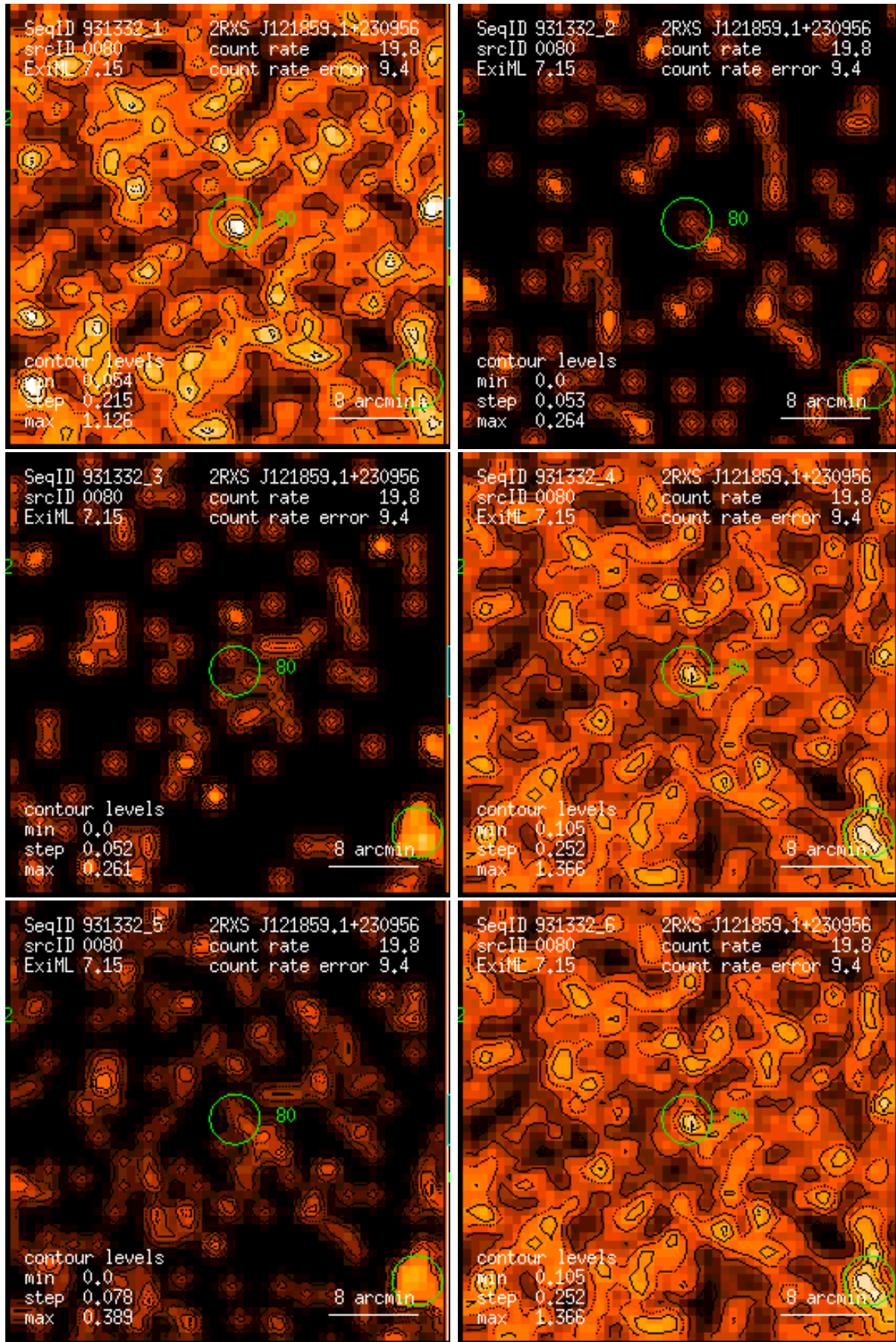
Figure 80: RASS 931332: detection 0080: band rate images, Gaussian filter: (1) PSPC channels 11 – 41, (2) 52 – 90, (3) 91 – 201, (4) 11 – 235, (5) 52 – 201, (6) 11 – 201. Broad band rates in counts/ks. Band rate contour levels in counts/ks/arcmin 2 .
