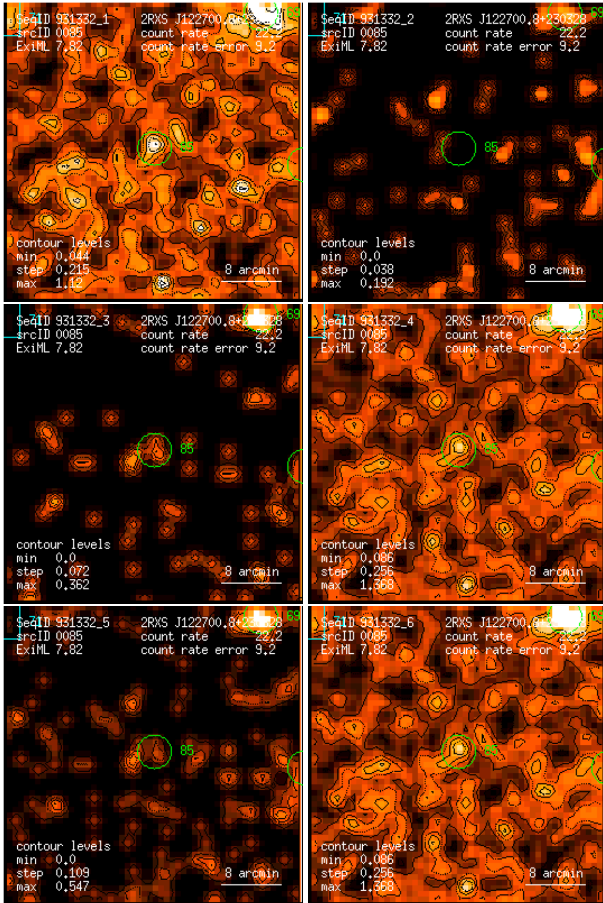
Figure 85: RASS 931332: detection 0085: band rate images, Gaussian filter: (1) PSPC channels 11 – 41, (2) 52 – 90, (3) 91 – 201, (4) 11 – 235, (5) 52 – 201, (6) 11 – 201. Broad band rates in counts/ks. Band rate contour levels in counts/ks/arcmin 2 .
