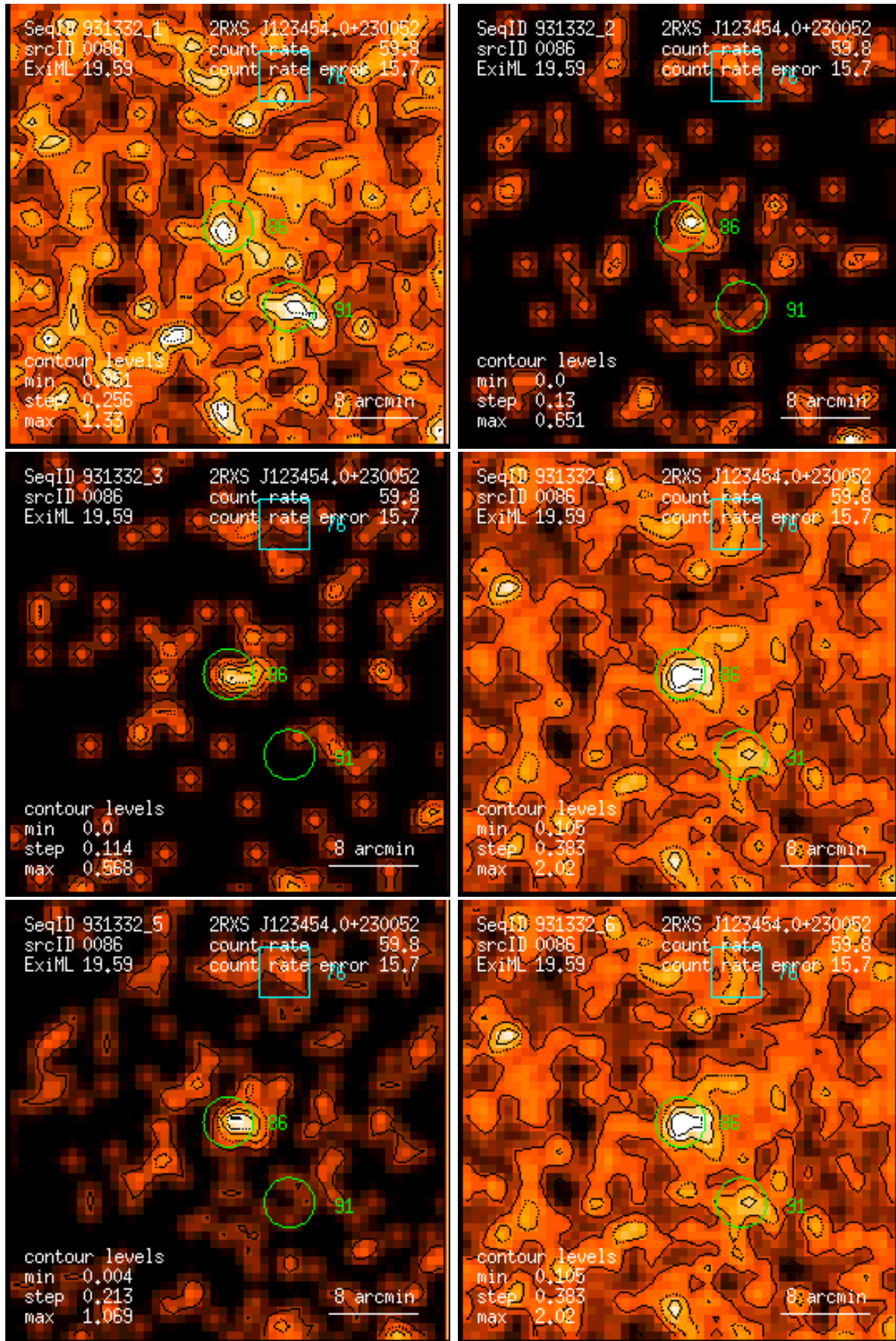
Figure 86: RASS 931332: detection 0086: band rate images, Gaussian filter: (1) PSPC channels 11 – 41, (2) 52 – 90, (3) 91 – 201, (4) 11 – 235, (5) 52 – 201, (6) 11 – 201. Broad band rates in counts/ks. Band rate contour levels in counts/ks/arcmin 2 .
