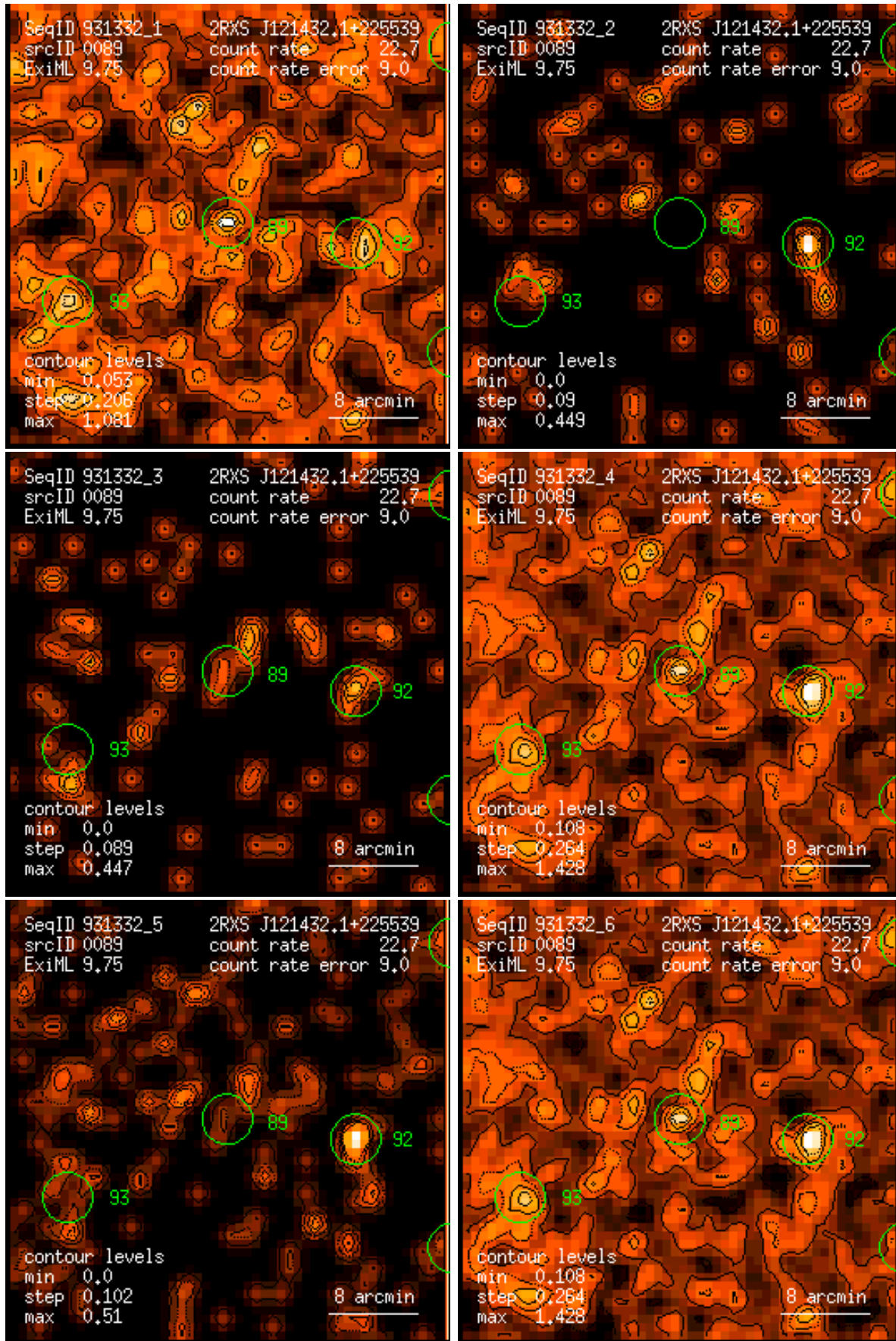
Figure 89: RASS 931332: detection 0089: band rate images, Gaussian filter: (1) PSPC channels 11 – 41, (2) 52 – 90, (3) 91 – 201, (4) 11 – 235, (5) 52 – 201, (6) 11 – 201. Broad band rates in counts/ks. Band rate contour levels in counts/ks/arcmin 2 .
