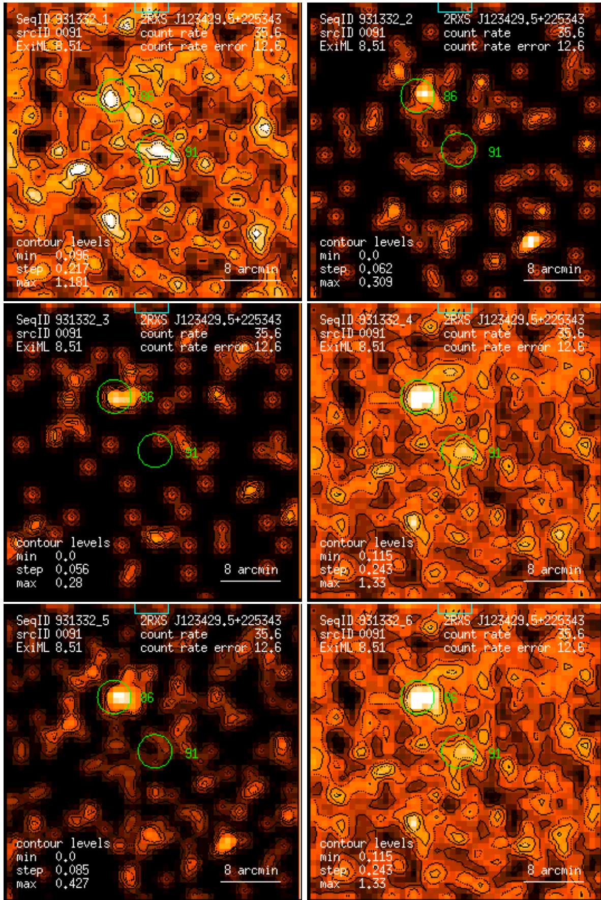
Figure 91: RASS 931332: detection 0091: band rate images, Gaussian filter: (1) PSPC channels 11 – 41, (2) 52 – 90, (3) 91 – 201, (4) 11 – 235, (5) 52 – 201, (6) 11 – 201. Broad band rates in counts/ks. Band rate contour levels in counts/ks/arcmin 2 .
