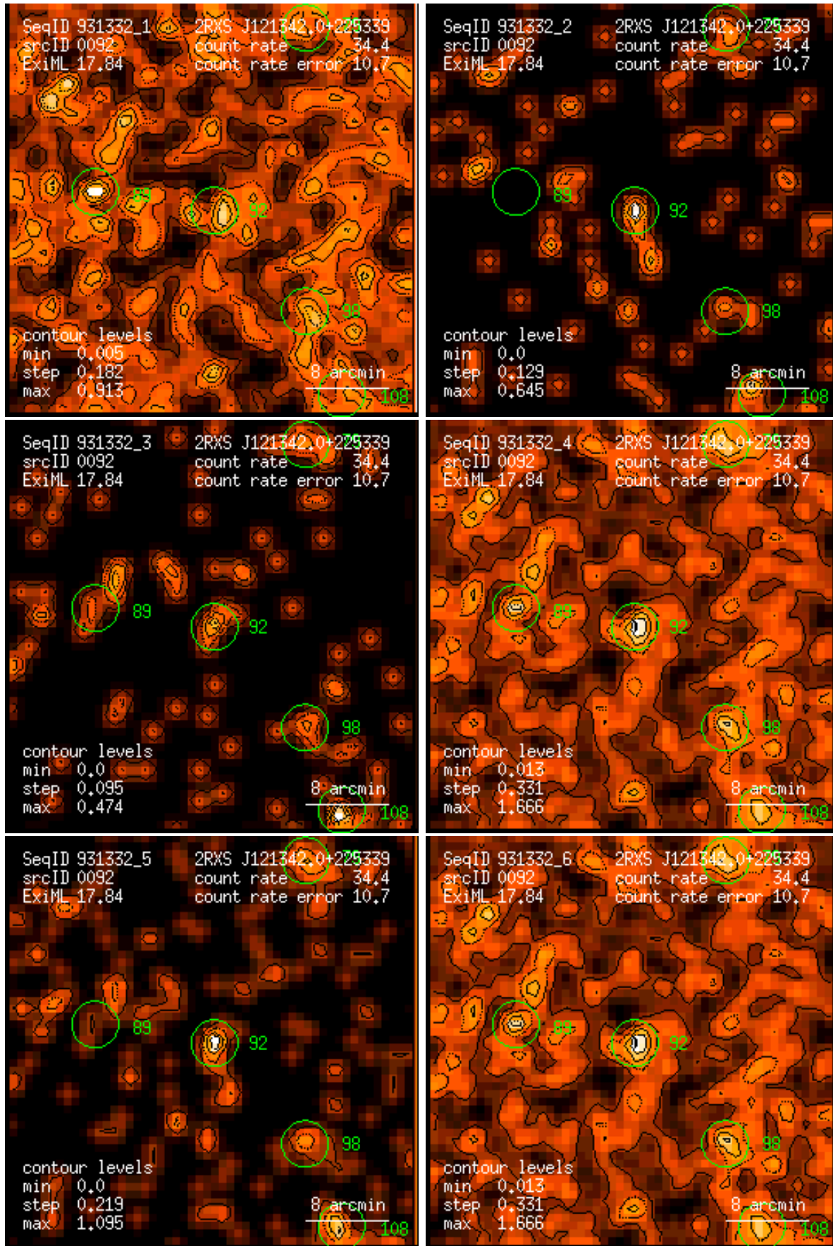
Figure 92: RASS 931332: detection 0092: band rate images, Gaussian filter: (1) PSPC channels 11 – 41, (2) 52 – 90, (3) 91 – 201, (4) 11 – 235, (5) 52 – 201, (6) 11 – 201. Broad band rates in counts/ks. Band rate contour levels in counts/ks/arcmin 2 .
