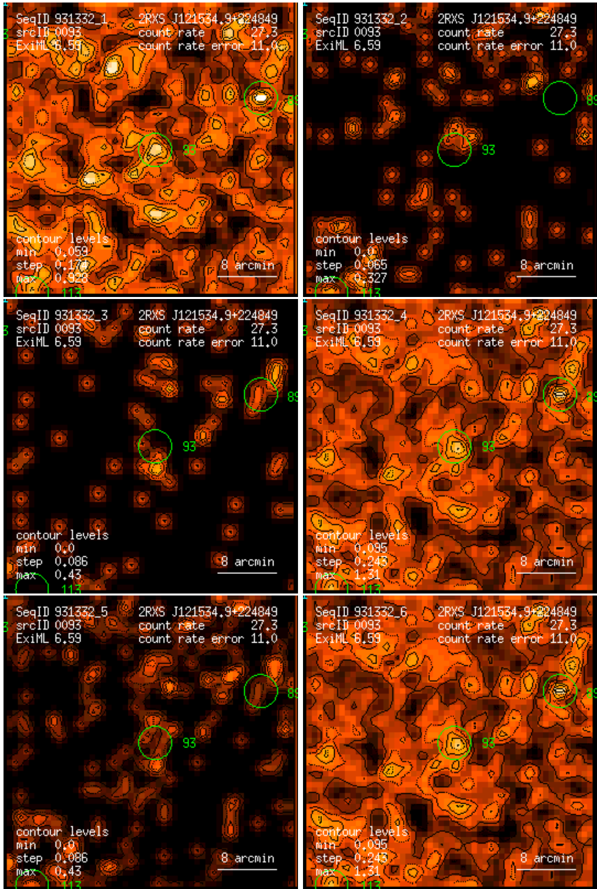
Figure 93: RASS 931332: detection 0093: band rate images, Gaussian filter: (1) PSPC channels 11 – 41, (2) 52 – 90, (3) 91 – 201, (4) 11 – 235, (5) 52 – 201, (6) 11 – 201. Broad band rates in counts/ks. Band rate contour levels in counts/ks/arcmin 2 .
