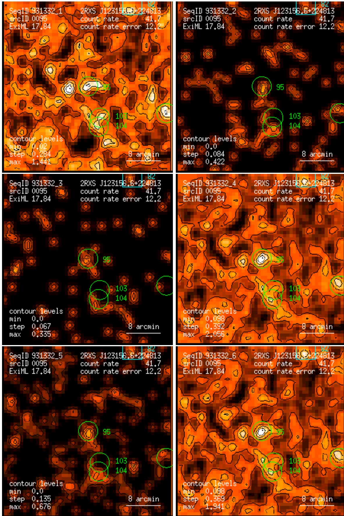
Figure 95: RASS 931332: detection 0095: band rate images, Gaussian filter: (1) PSPC channels 11 – 41, (2) 52 – 90, (3) 91 – 201, (4) 11 – 235, (5) 52 – 201, (6) 11 – 201. Broad band rates in counts/ks. Band rate contour levels in counts/ks/arcmin 2 .
