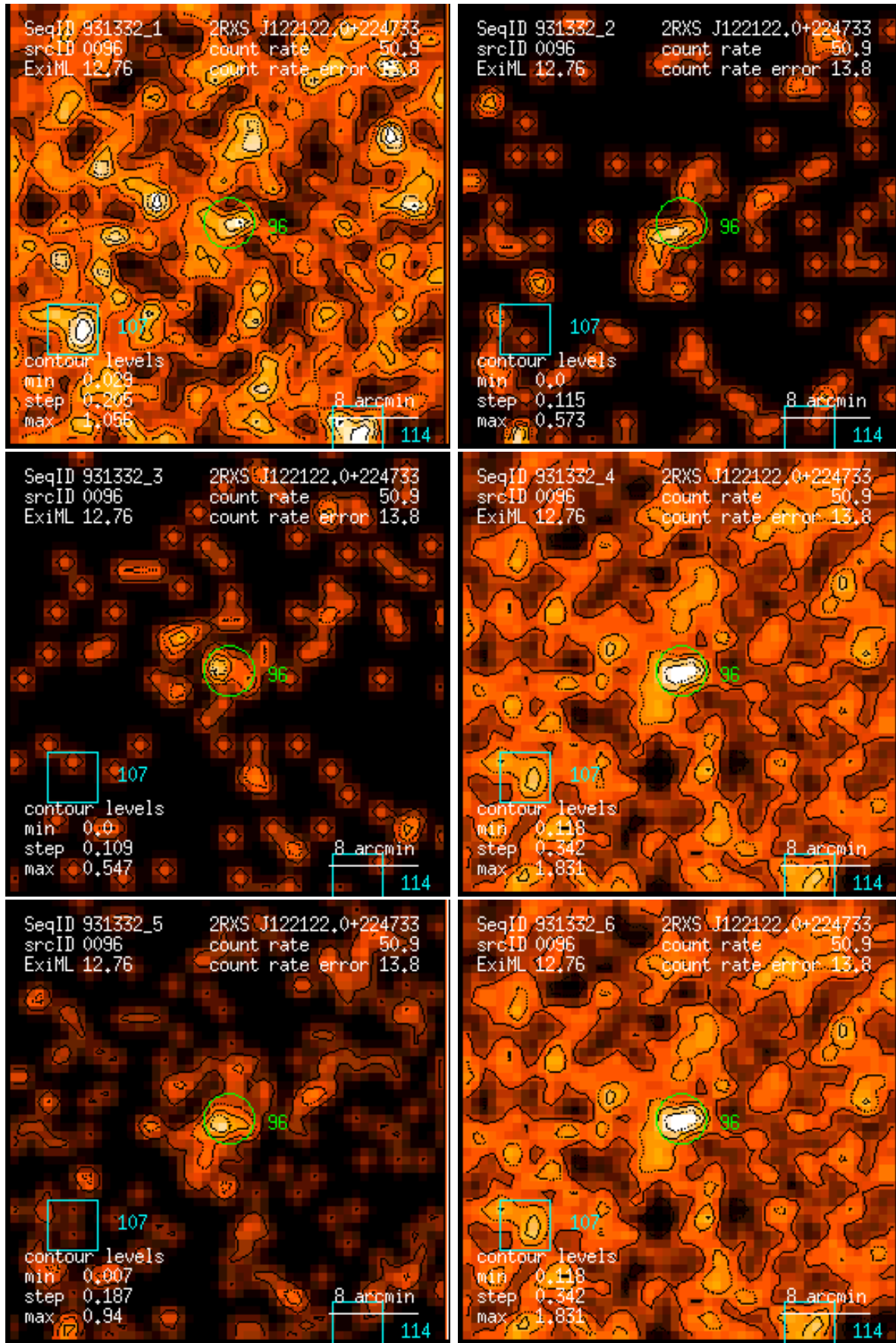
Figure 96: RASS 931332: detection 0096: band rate images, Gaussian filter: (1) PSPC channels 11 – 41, (2) 52 – 90, (3) 91 – 201, (4) 11 – 235, (5) 52 – 201, (6) 11 – 201. Broad band rates in counts/ks. Band rate contour levels in counts/ks/arcmin 2 .
