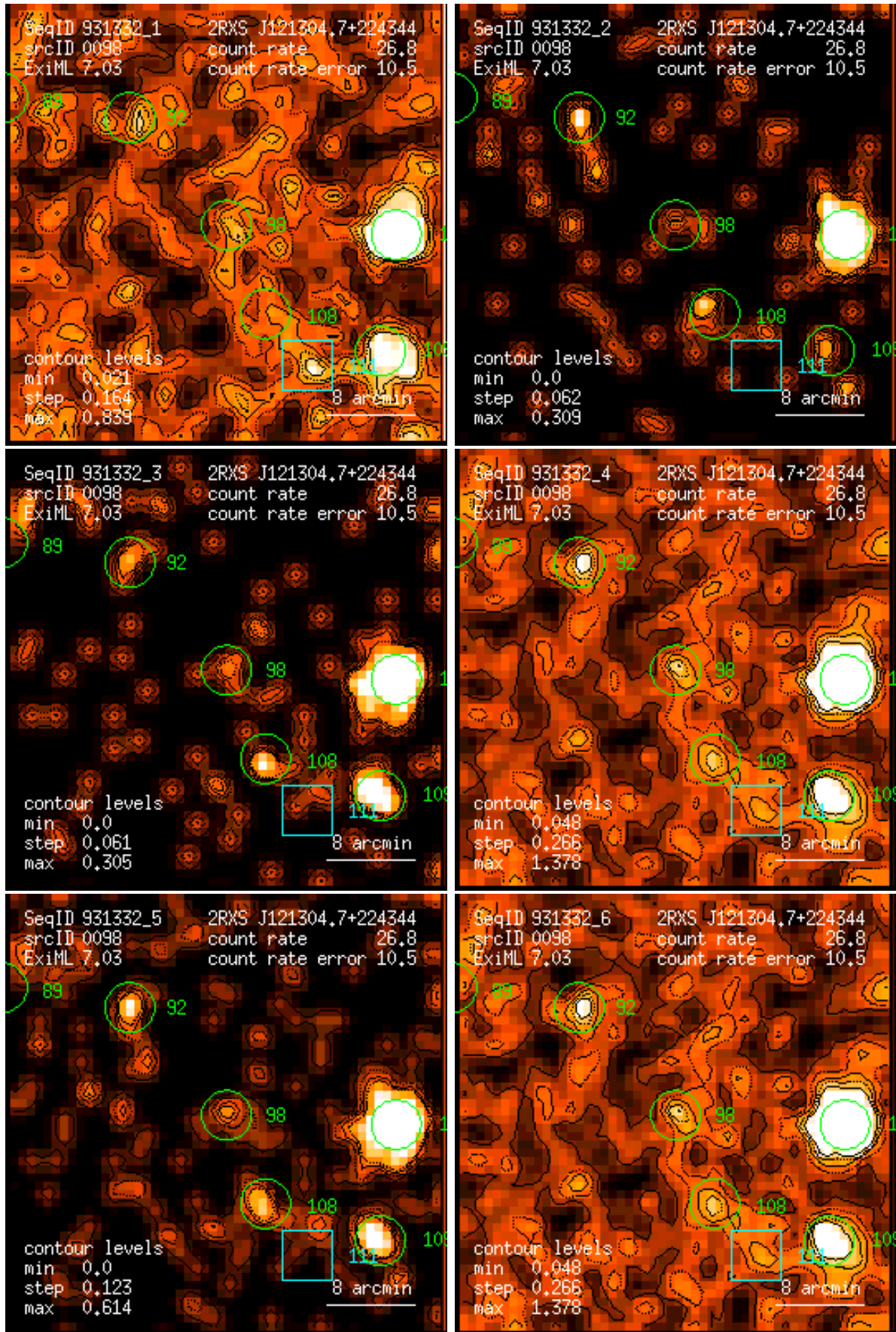
Figure 98: RASS 931332: detection 0098: band rate images, Gaussian filter: (1) PSPC channels 11 – 41, (2) 52 – 90, (3) 91 – 201, (4) 11 – 235, (5) 52 – 201, (6) 11 – 201. Broad band rates in counts/ks. Band rate contour levels in counts/ks/arcmin 2 .
