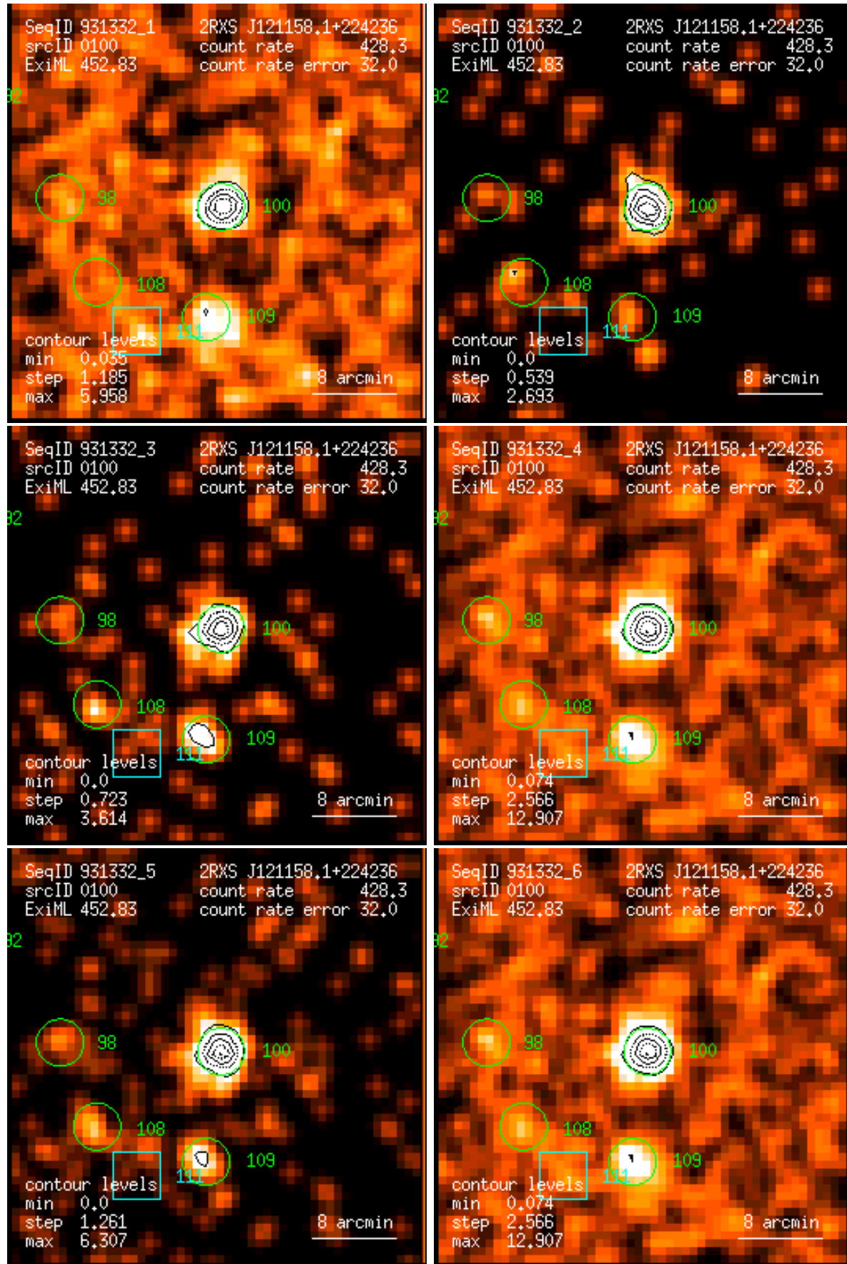
Figure 100: RASS 931332: detection 0100: band rate images, Gaussian filter: (1) PSPC channels 11 – 41, (2) 52 – 90, (3) 91 – 201, (4) 11 – 235, (5) 52 – 201, (6) 11 – 201. Broad band rates in counts/ks. Band rate contour levels in counts/ks/arcmin 2 .
