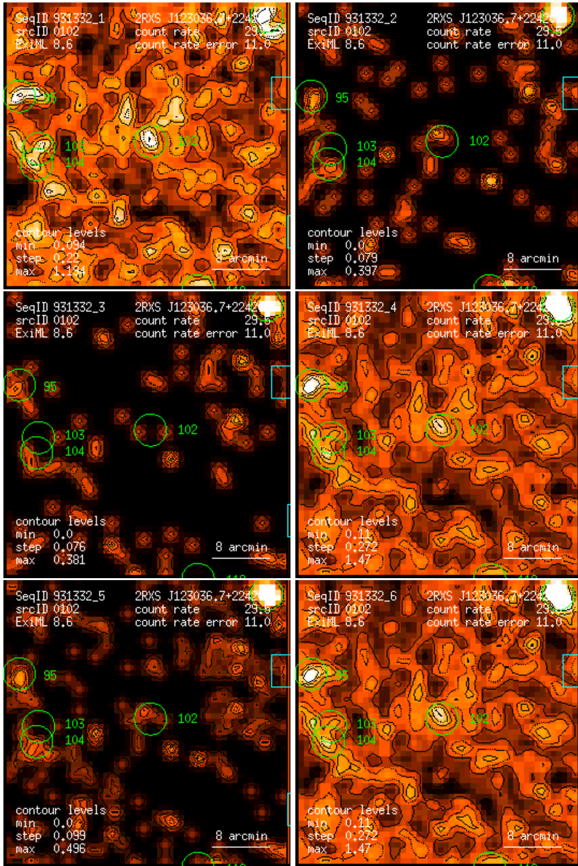
Figure 102: RASS 931332: detection 0102: band rate images, Gaussian filter: (1) PSPC channels 11 – 41, (2) 52 – 90, (3) 91 – 201, (4) 11 – 235, (5) 52 – 201, (6) 11 – 201. Broad band rates in counts/ks. Band rate contour levels in counts/ks/arcmin 2 .
