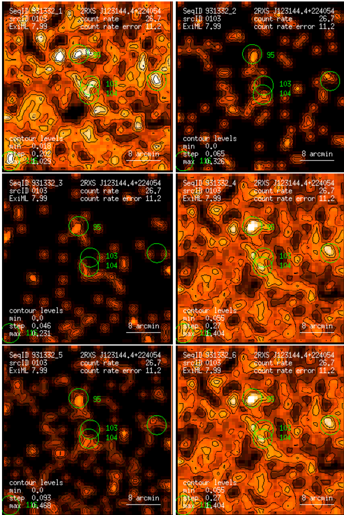
Figure 103: RASS 931332: detection 0103: band rate images, Gaussian filter: (1) PSPC channels 11 – 41, (2) 52 – 90, (3) 91 – 201, (4) 11 – 235, (5) 52 – 201, (6) 11 – 201. Broad band rates in counts/ks. Band rate contour levels in counts/ks/arcmin 2 .
