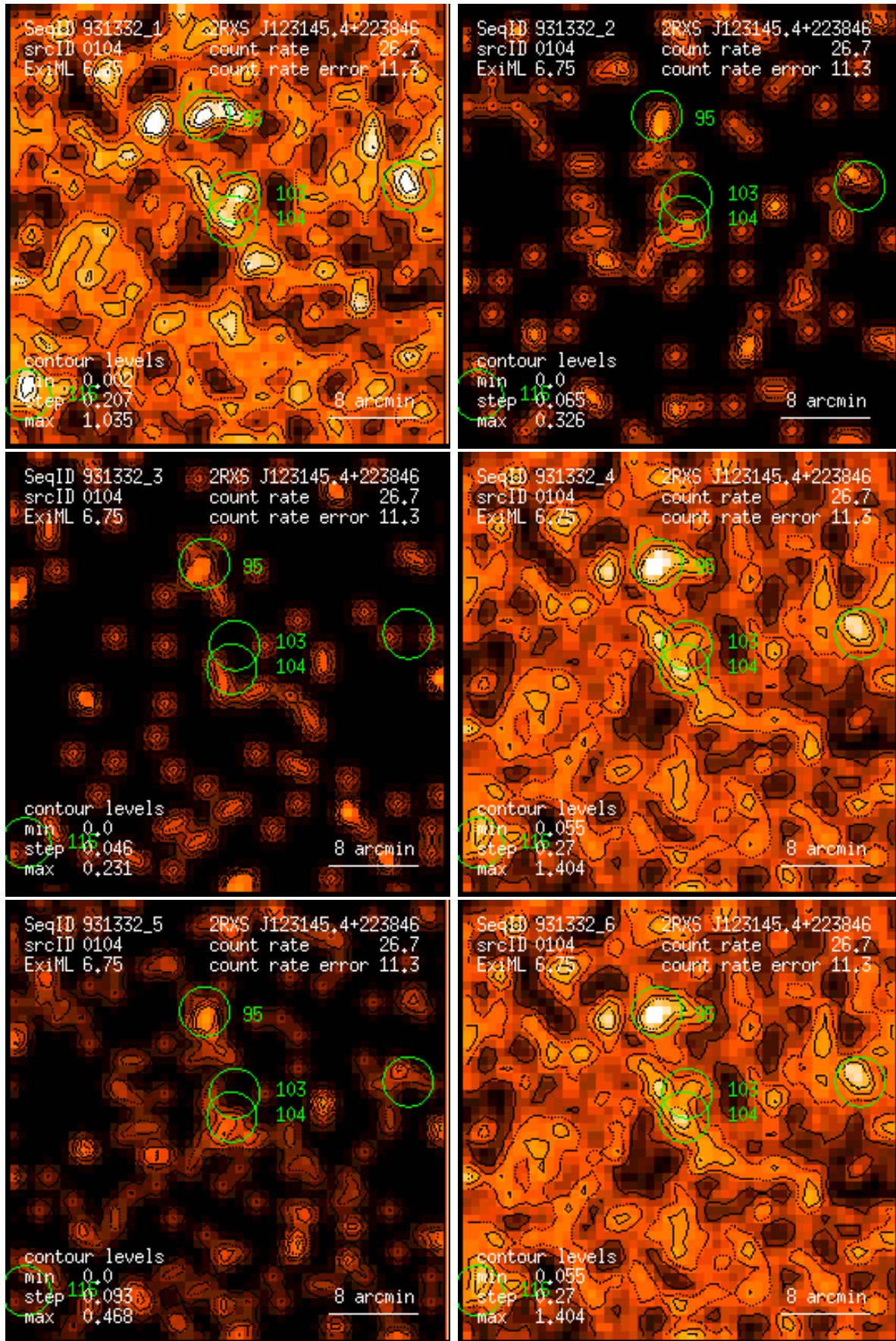
Figure 104: RASS 931332: detection 0104: band rate images, Gaussian filter: (1) PSPC channels 11 – 41, (2) 52 – 90, (3) 91 – 201, (4) 11 – 235, (5) 52 – 201, (6) 11 – 201. Broad band rates in counts/ks. Band rate contour levels in counts/ks/arcmin 2 .
