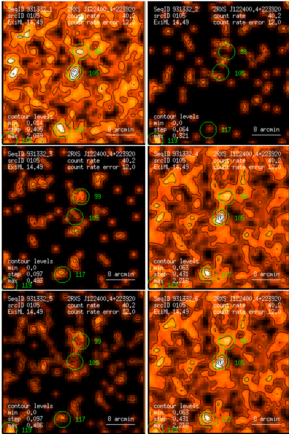
Figure 105: RASS 931332: detection 0105: band rate images, Gaussian filter: (1) PSPC channels 11 – 41, (2) 52 – 90, (3) 91 – 201, (4) 11 – 235, (5) 52 – 201, (6) 11 – 201. Broad band rates in counts/ks. Band rate contour levels in counts/ks/arcmin 2 .
