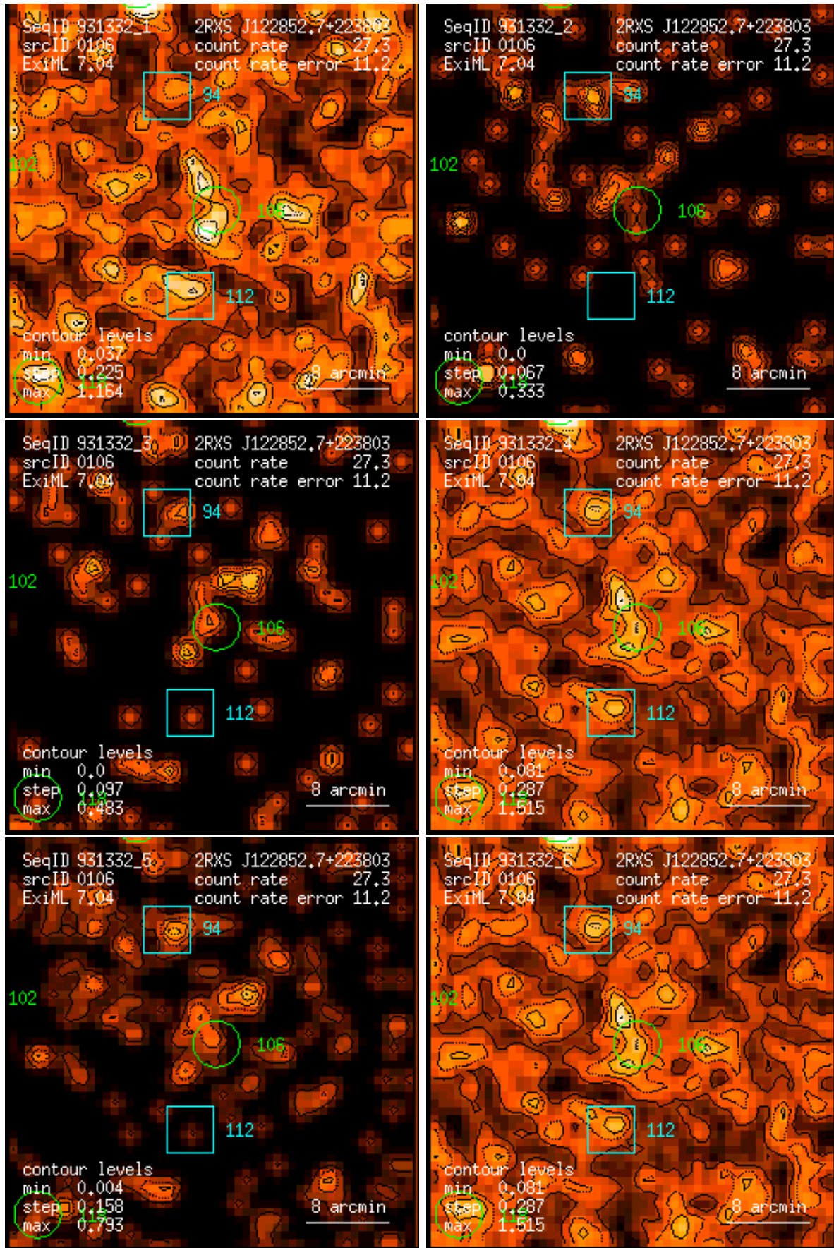
Figure 106: RASS 931332: detection 0106: band rate images, Gaussian filter: (1) PSPC channels 11 – 41, (2) 52 – 90, (3) 91 – 201, (4) 11 – 235, (5) 52 – 201, (6) 11 – 201. Broad band rates in counts/ks. Band rate contour levels in counts/ks/arcmin 2 .
