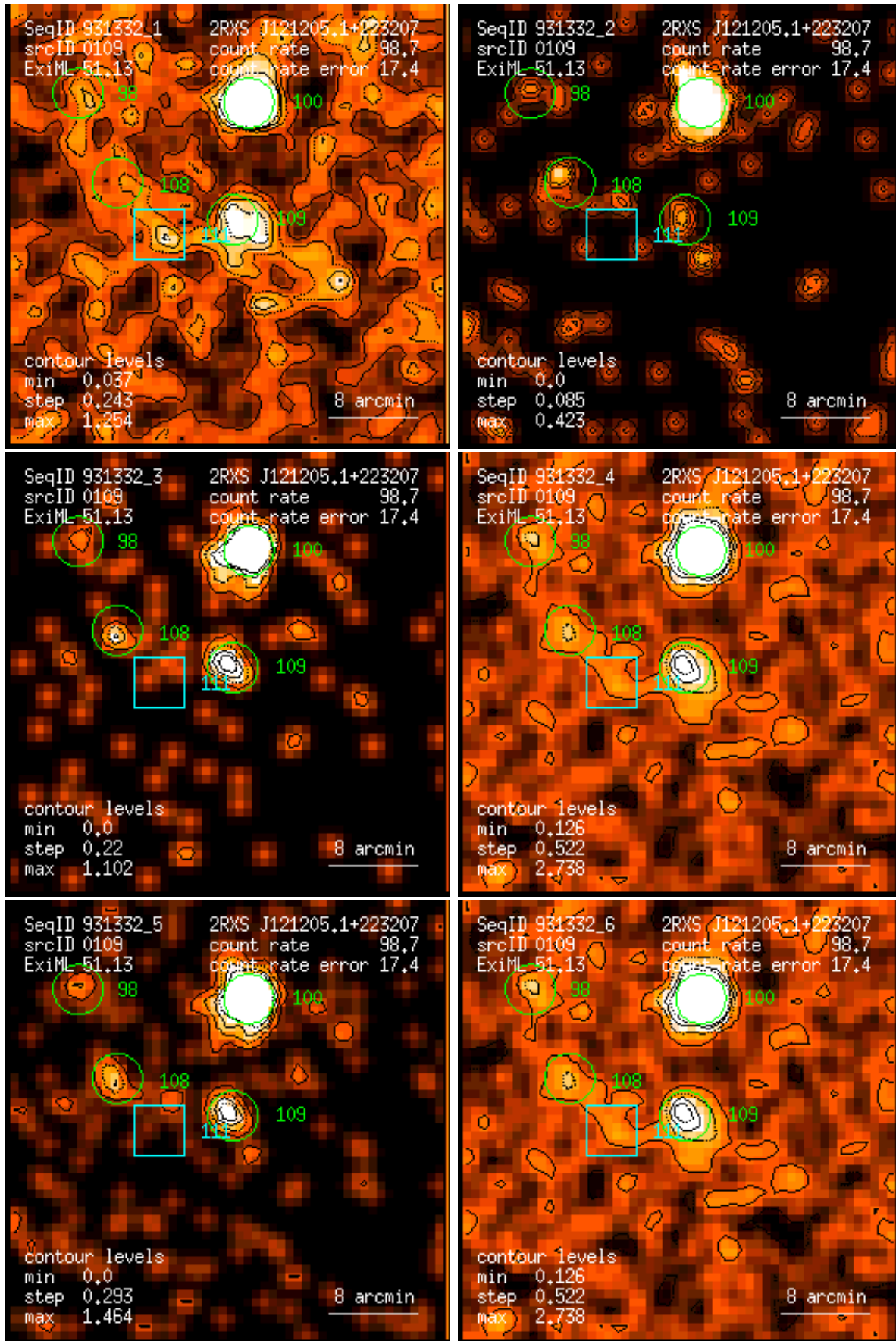
Figure 109: RASS 931332: detection 0109: band rate images, Gaussian filter: (1) PSPC channels 11 – 41, (2) 52 – 90, (3) 91 – 201, (4) 11 – 235, (5) 52 – 201, (6) 11 – 201. Broad band rates in counts/ks. Band rate contour levels in counts/ks/arcmin 2 .
