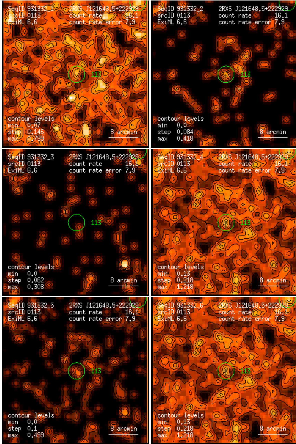
Figure 113: RASS 931332: detection 0113: band rate images, Gaussian filter: (1) PSPC channels 11 – 41, (2) 52 – 90, (3) 91 – 201, (4) 11 – 235, (5) 52 – 201, (6) 11 – 201. Broad band rates in counts/ks. Band rate contour levels in counts/ks/arcmin 2 .
