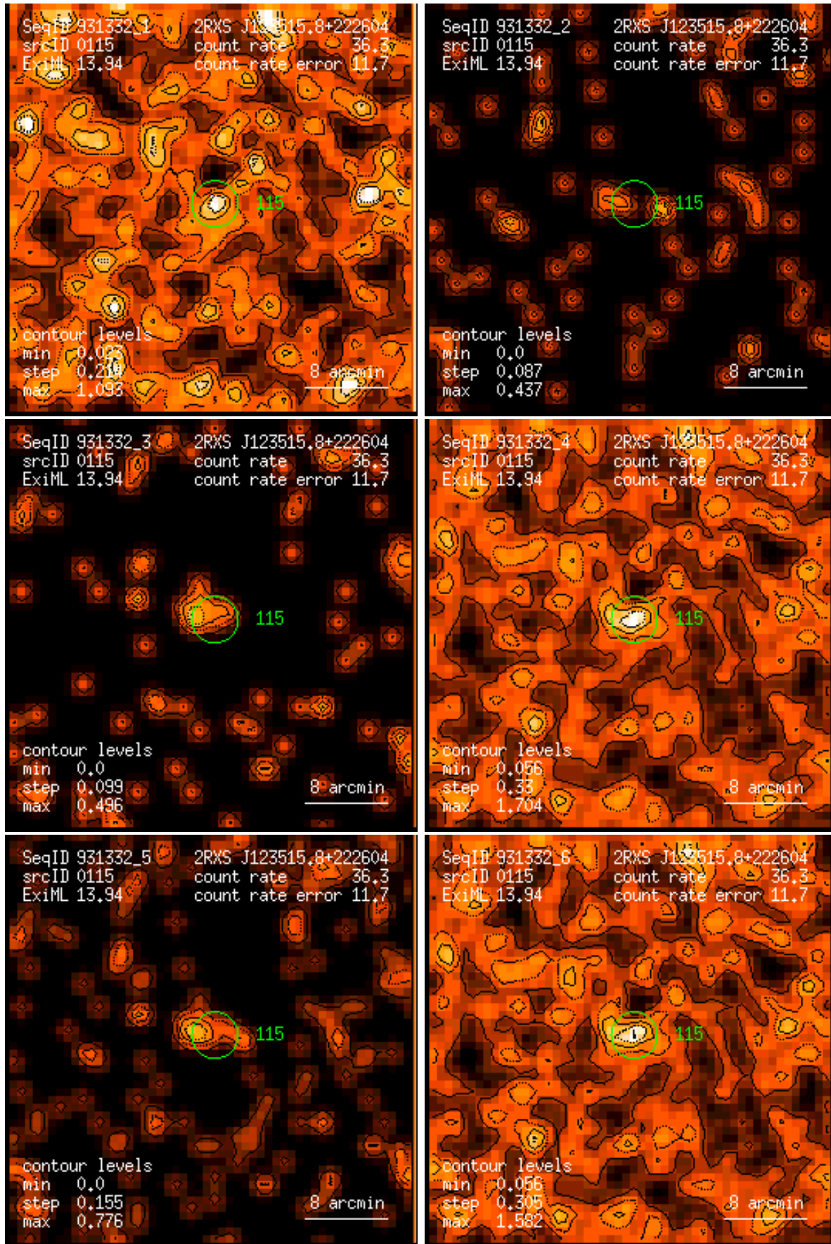
Figure 115: RASS 931332: detection 0115: band rate images, Gaussian filter: (1) PSPC channels 11 – 41, (2) 52 – 90, (3) 91 – 201, (4) 11 – 235, (5) 52 – 201, (6) 11 – 201. Broad band rates in counts/ks. Band rate contour levels in counts/ks/arcmin 2 .
