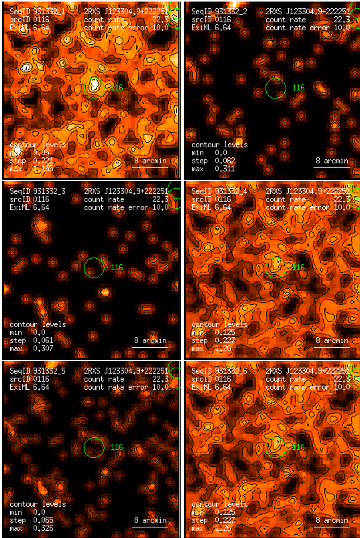
Figure 116: RASS 931332: detection 0116: band rate images, Gaussian filter: (1) PSPC channels 11 – 41, (2) 52 – 90, (3) 91 – 201, (4) 11 – 235, (5) 52 – 201, (6) 11 – 201. Broad band rates in counts/ks. Band rate contour levels in counts/ks/arcmin 2 .
