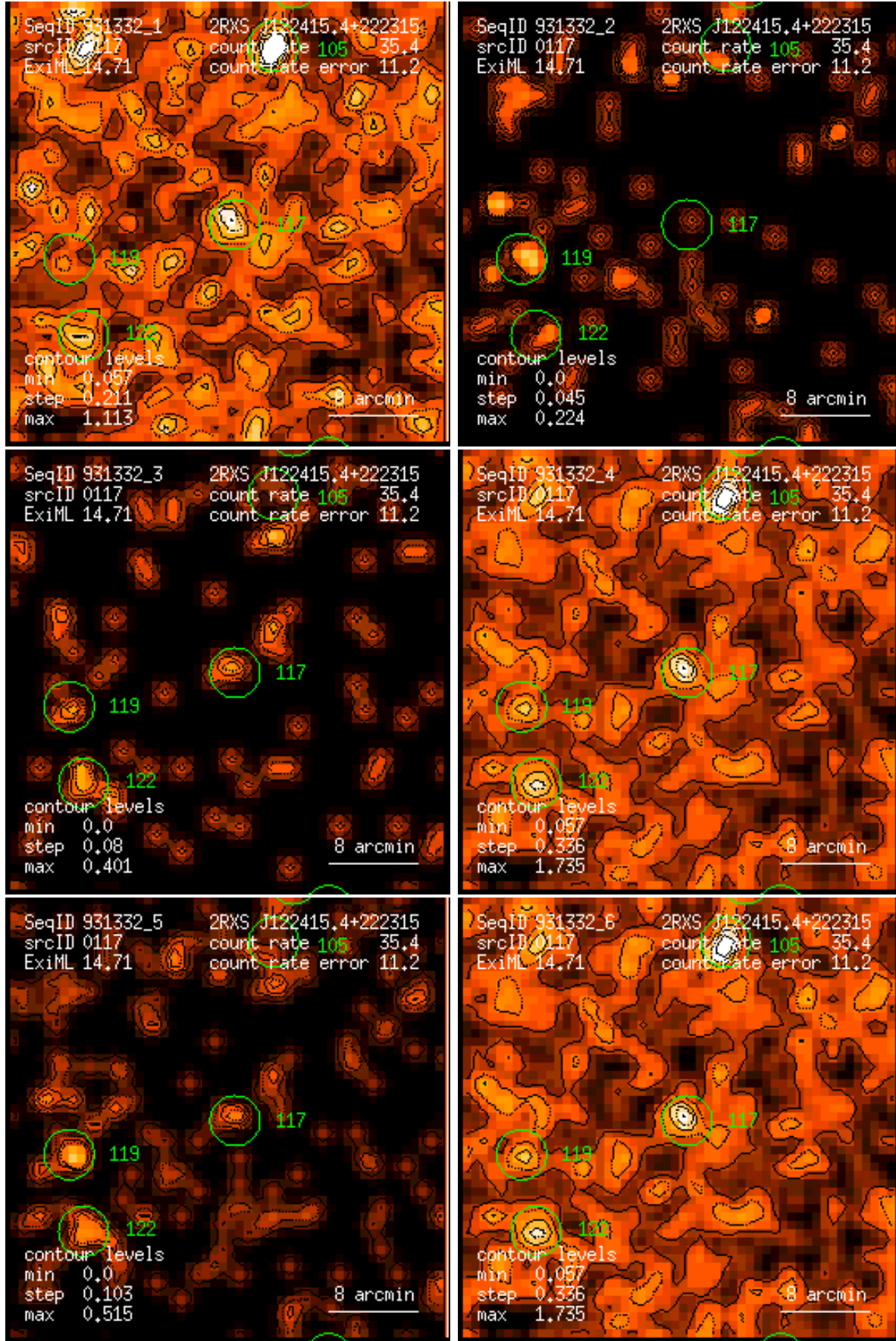
Figure 117: RASS 931332: detection 0117: band rate images, Gaussian filter: (1) PSPC channels 11 – 41, (2) 52 – 90, (3) 91 – 201, (4) 11 – 235, (5) 52 – 201, (6) 11 – 201. Broad band rates in counts/ks. Band rate contour levels in counts/ks/arcmin 2 .
