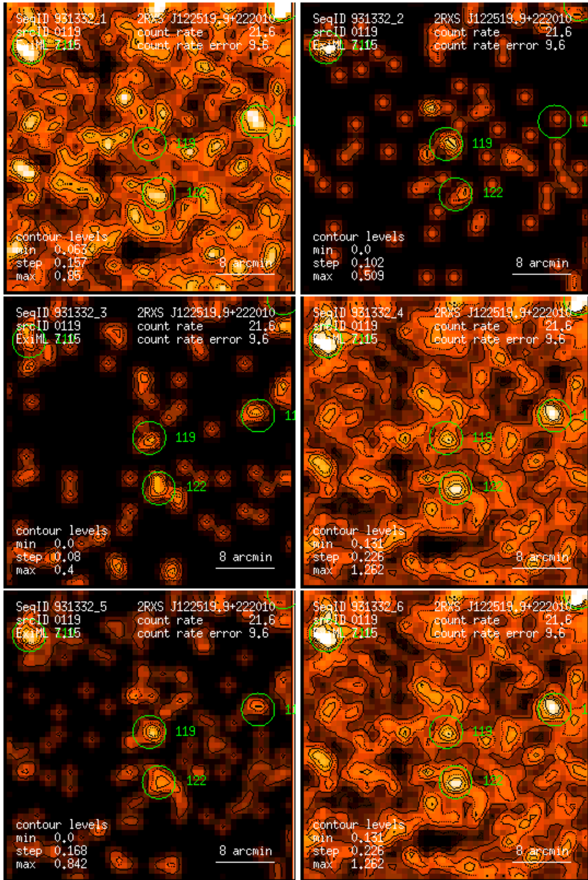
Figure 119: RASS 931332: detection 0119: band rate images, Gaussian filter: (1) PSPC channels 11 – 41, (2) 52 – 90, (3) 91 – 201, (4) 11 – 235, (5) 52 – 201, (6) 11 – 201. Broad band rates in counts/ks. Band rate contour levels in counts/ks/arcmin 2 .
