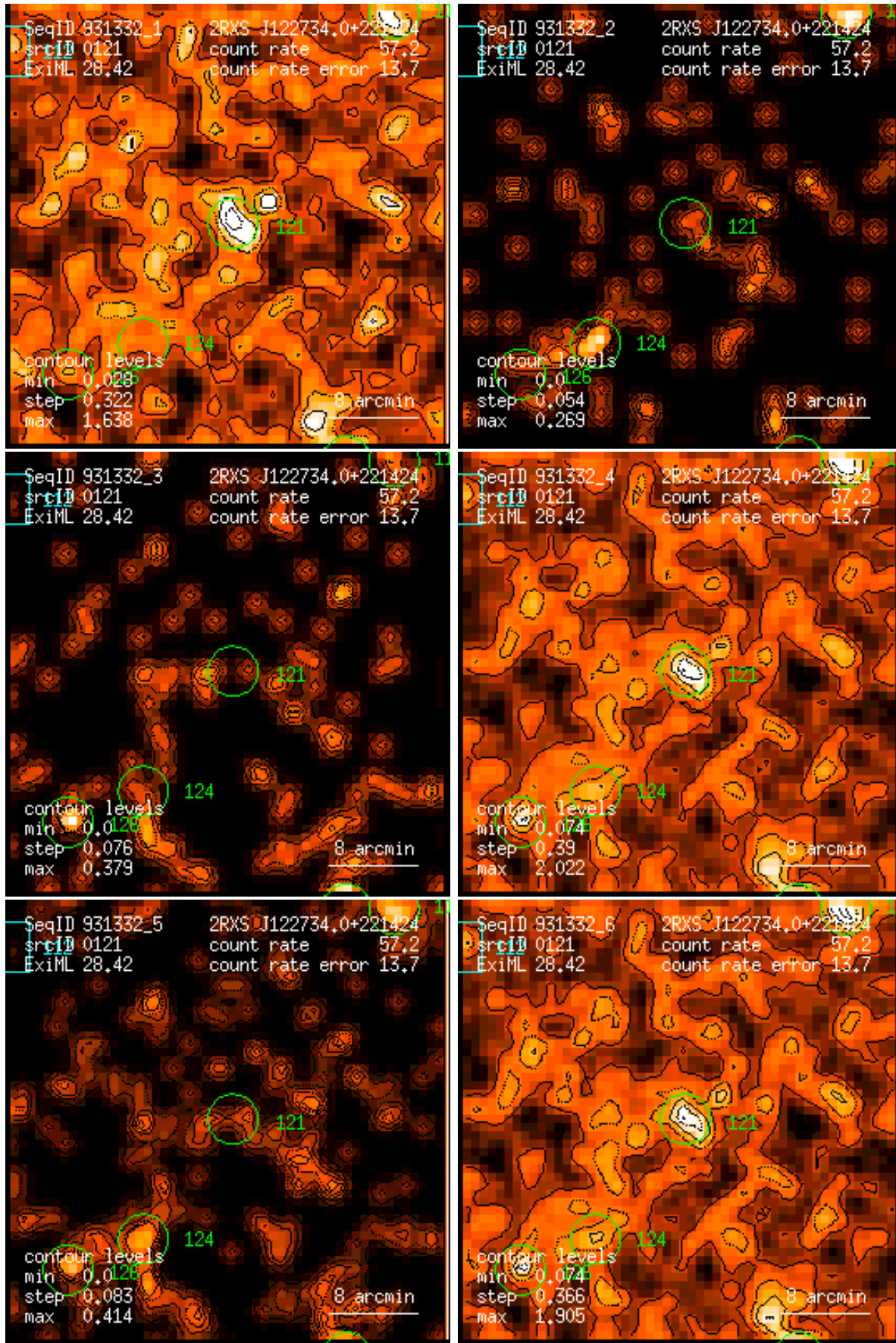
Figure 121: RASS 931332: detection 0121: band rate images, Gaussian filter: (1) PSPC channels 11 – 41, (2) 52 – 90, (3) 91 – 201, (4) 11 – 235, (5) 52 – 201, (6) 11 – 201. Broad band rates in counts/ks. Band rate contour levels in counts/ks/arcmin 2 .
