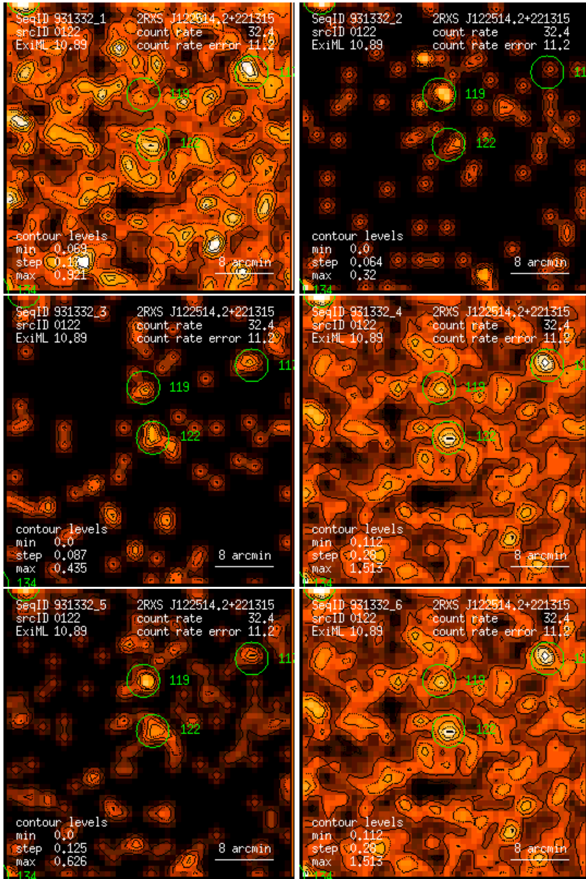
Figure 122: RASS 931332: detection 0122: band rate images, Gaussian filter: (1) PSPC channels 11 – 41, (2) 52 – 90, (3) 91 – 201, (4) 11 – 235, (5) 52 – 201, (6) 11 – 201. Broad band rates in counts/ks. Band rate contour levels in counts/ks/arcmin 2 .
