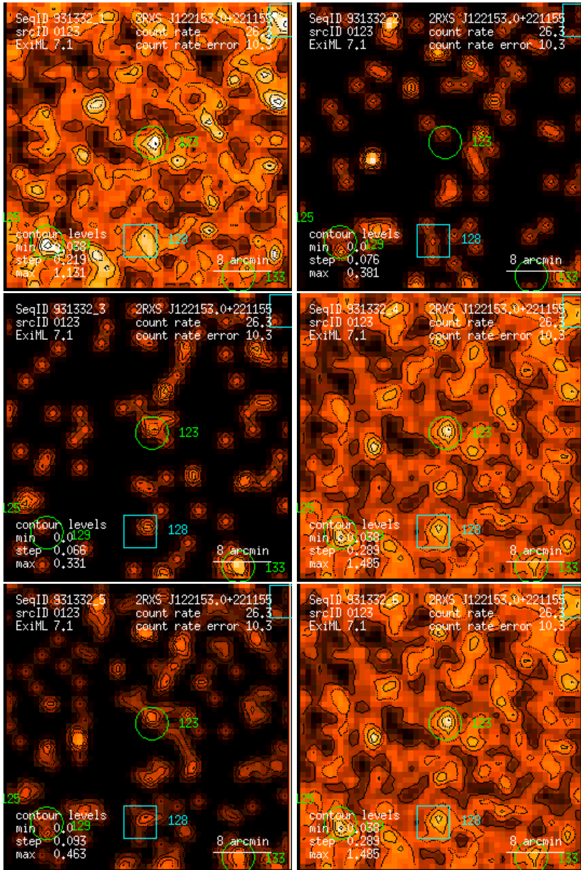
Figure 123: RASS 931332: detection 0123: band rate images, Gaussian filter: (1) PSPC channels 11 – 41, (2) 52 – 90, (3) 91 – 201, (4) 11 – 235, (5) 52 – 201, (6) 11 – 201. Broad band rates in counts/ks. Band rate contour levels in counts/ks/arcmin 2 .
