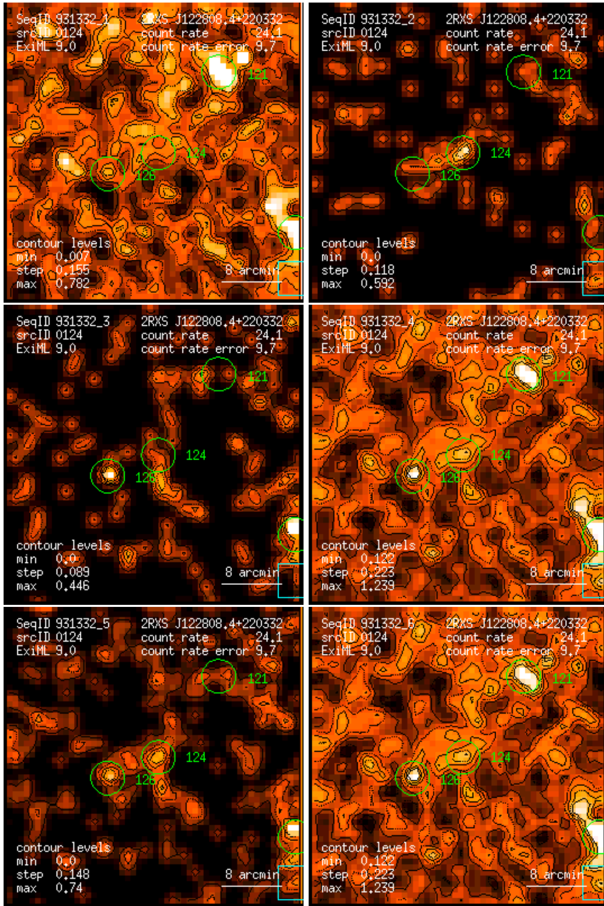
Figure 124: RASS 931332: detection 0124: band rate images, Gaussian filter: (1) PSPC channels 11 – 41, (2) 52 – 90, (3) 91 – 201, (4) 11 – 235, (5) 52 – 201, (6) 11 – 201. Broad band rates in counts/ks. Band rate contour levels in counts/ks/arcmin 2 .
