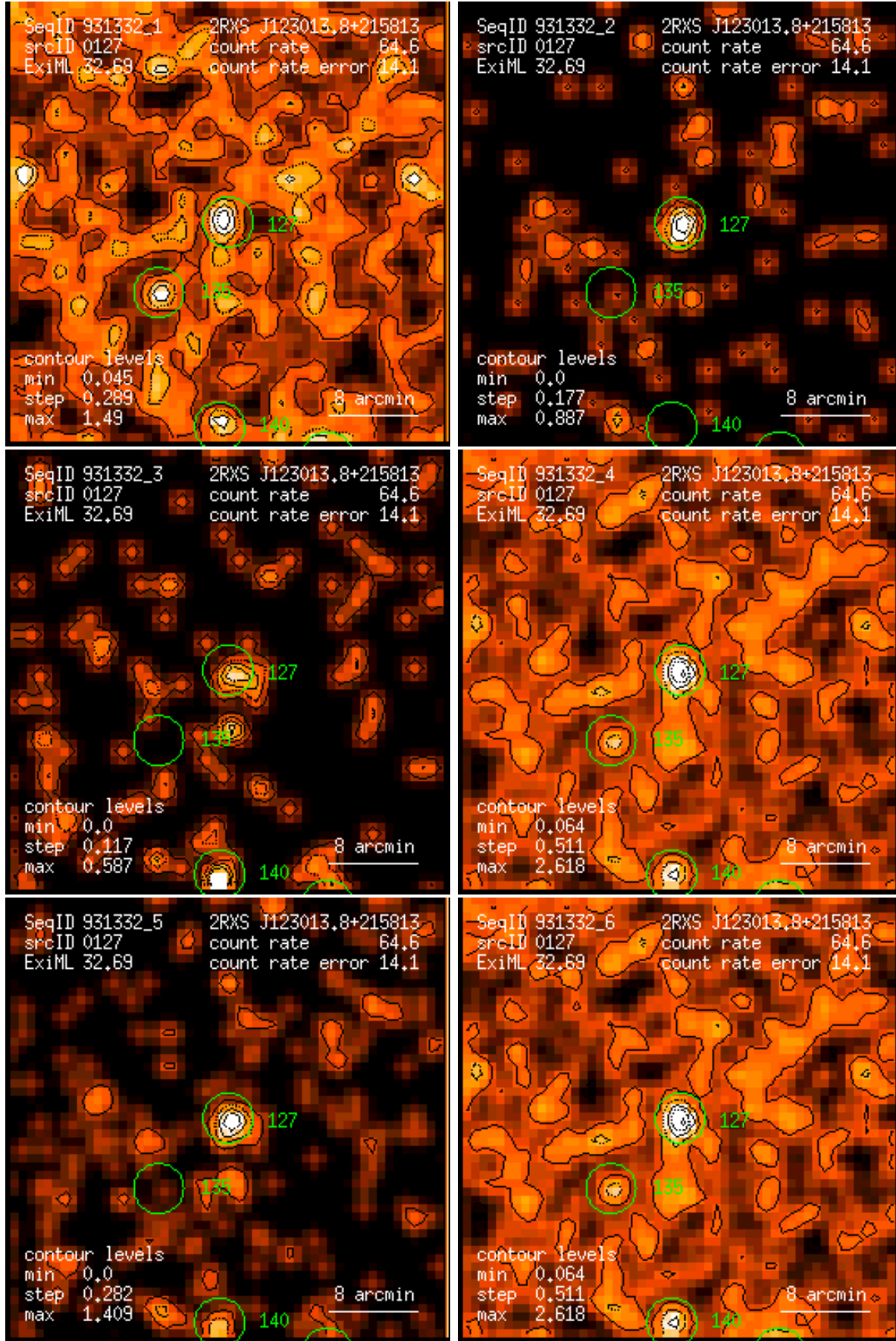
Figure 127: RASS 931332: detection 0127: band rate images, Gaussian filter: (1) PSPC channels 11 – 41, (2) 52 – 90, (3) 91 – 201, (4) 11 – 235, (5) 52 – 201, (6) 11 – 201. Broad band rates in counts/ks. Band rate contour levels in counts/ks/arcmin 2 .
