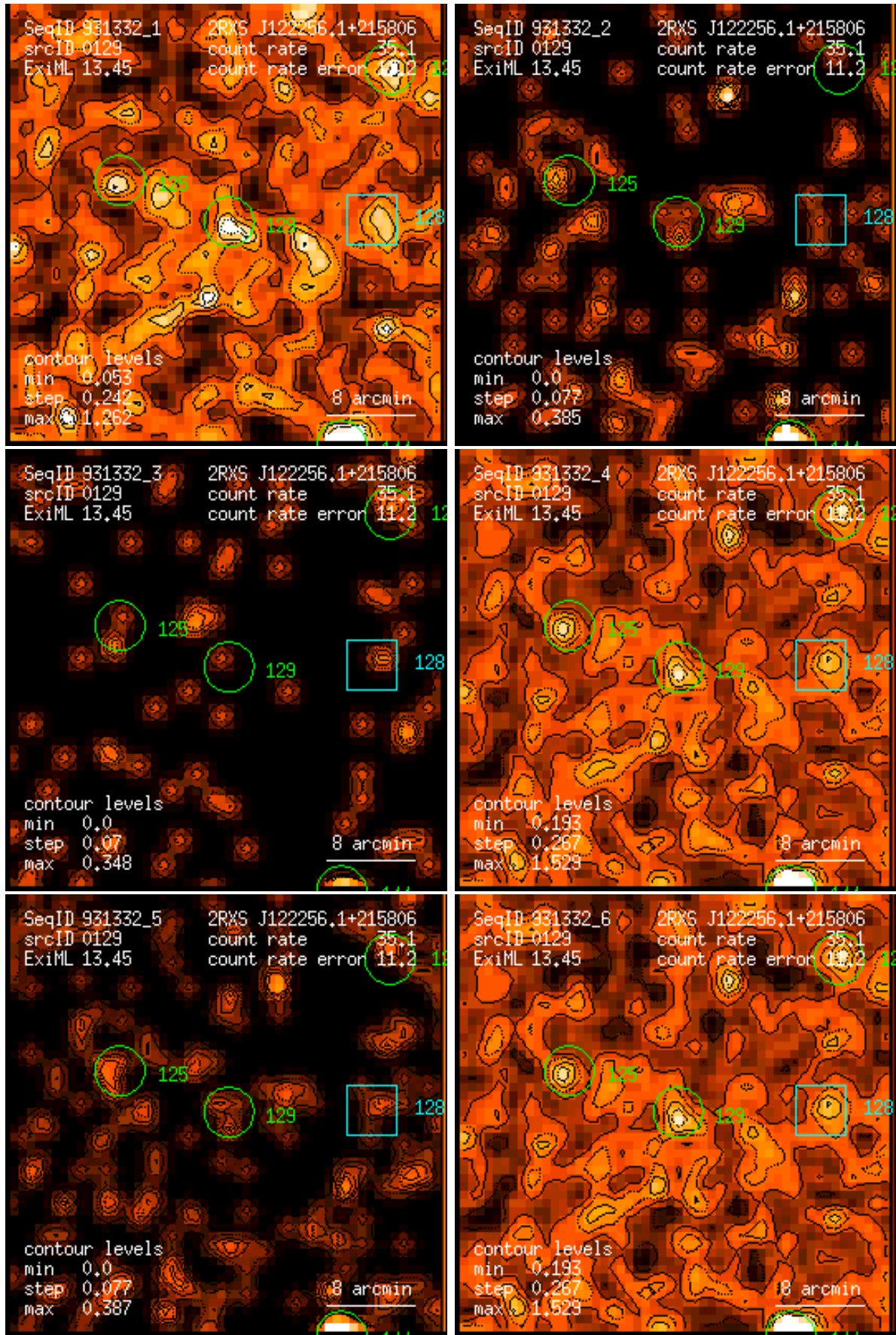
Figure 129: RASS 931332: detection 0129: band rate images, Gaussian filter: (1) PSPC channels 11 – 41, (2) 52 – 90, (3) 91 – 201, (4) 11 – 235, (5) 52 – 201, (6) 11 – 201. Broad band rates in counts/ks. Band rate contour levels in counts/ks/arcmin 2 .
