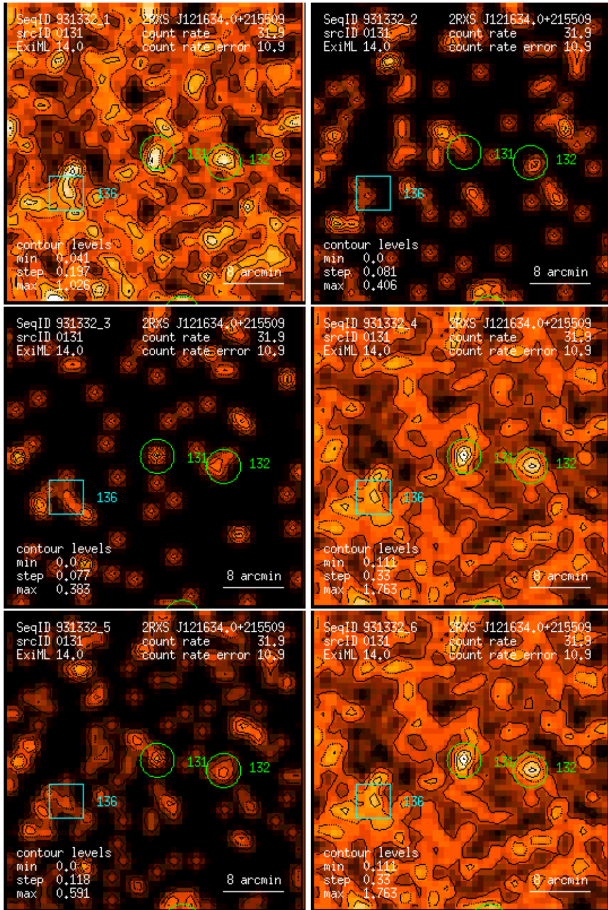
Figure 131: RASS 931332: detection 0131: band rate images, Gaussian filter: (1) PSPC channels 11 – 41, (2) 52 – 90, (3) 91 – 201, (4) 11 – 235, (5) 52 – 201, (6) 11 – 201. Broad band rates in counts/ks. Band rate contour levels in counts/ks/arcmin 2 .
