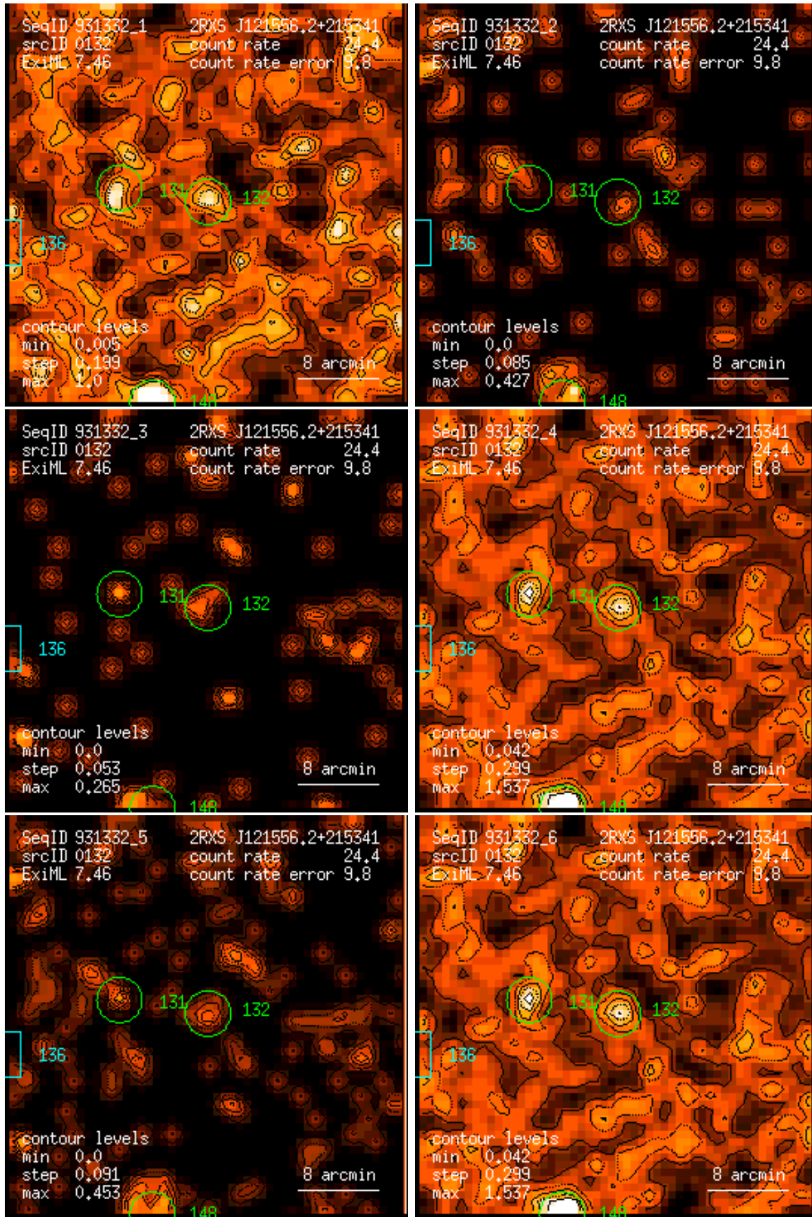
Figure 132: RASS 931332: detection 0132: band rate images, Gaussian filter: (1) PSPC channels 11 – 41, (2) 52 – 90, (3) 91 – 201, (4) 11 – 235, (5) 52 – 201, (6) 11 – 201. Broad band rates in counts/ks. Band rate contour levels in counts/ks/arcmin 2 .
