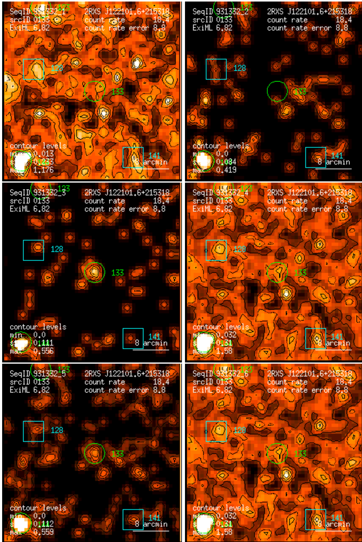
Figure 133: RASS 931332: detection 0133: band rate images, Gaussian filter: (1) PSPC channels 11 – 41, (2) 52 – 90, (3) 91 – 201, (4) 11 – 235, (5) 52 – 201, (6) 11 – 201. Broad band rates in counts/ks. Band rate contour levels in counts/ks/arcmin 2 .
