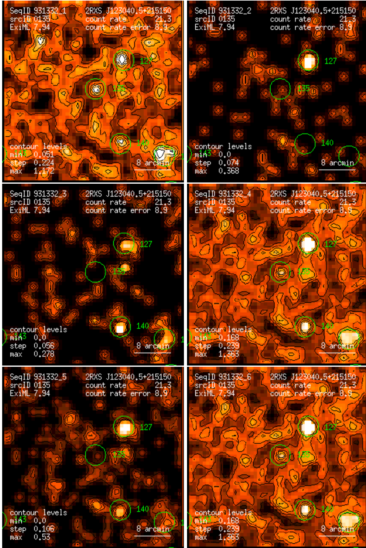
Figure 135: RASS 931332: detection 0135: band rate images, Gaussian filter: (1) PSPC channels 11 – 41, (2) 52 – 90, (3) 91 – 201, (4) 11 – 235, (5) 52 – 201, (6) 11 – 201. Broad band rates in counts/ks. Band rate contour levels in counts/ks/arcmin 2 .
