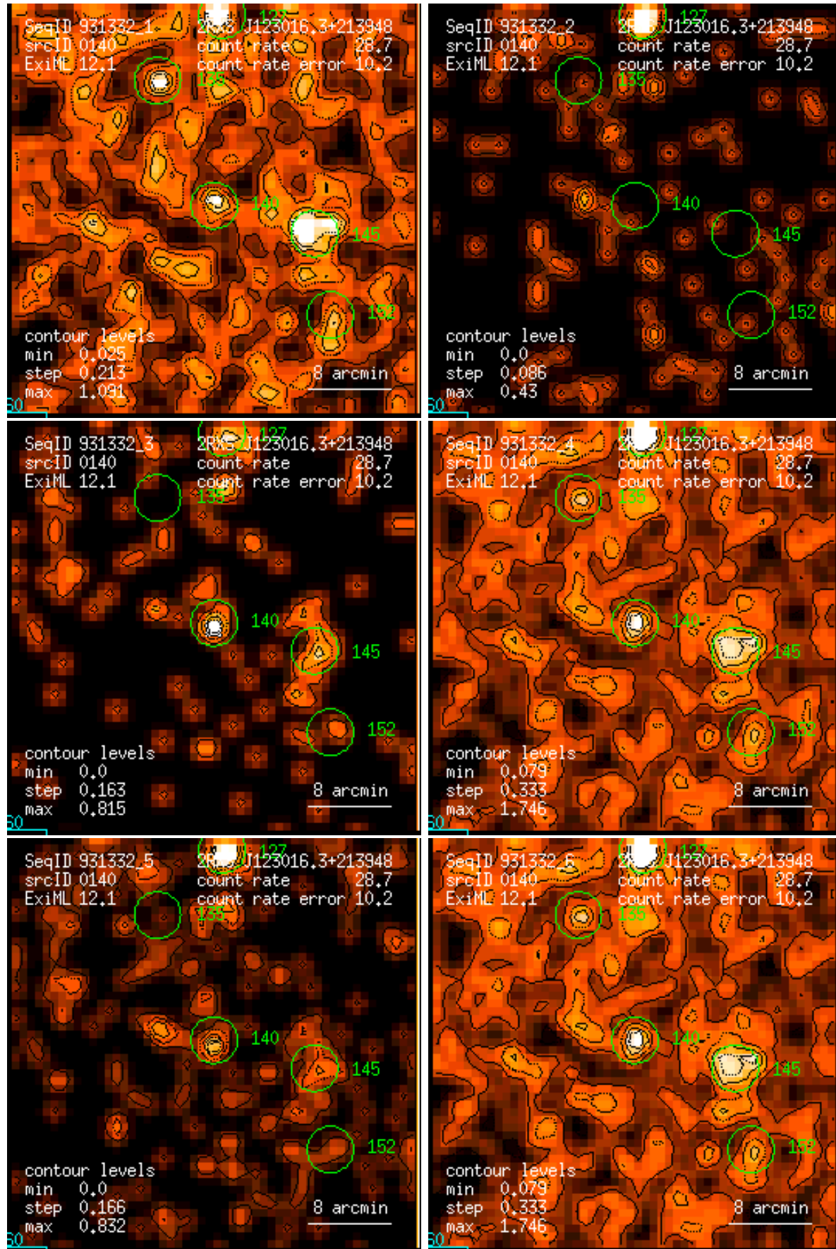
Figure 140: RASS 931332: detection 0140: band rate images, Gaussian filter: (1) PSPC channels 11 – 41, (2) 52 – 90, (3) 91 – 201, (4) 11 – 235, (5) 52 – 201, (6) 11 – 201. Broad band rates in counts/ks. Band rate contour levels in counts/ks/arcmin 2 .
