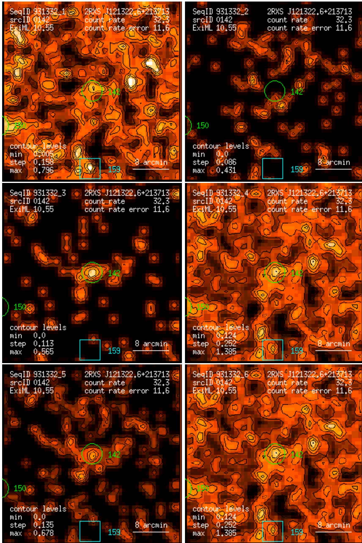
Figure 142: RASS 931332: detection 0142: band rate images, Gaussian filter: (1) PSPC channels 11 – 41, (2) 52 – 90, (3) 91 – 201, (4) 11 – 235, (5) 52 – 201, (6) 11 – 201. Broad band rates in counts/ks. Band rate contour levels in counts/ks/arcmin 2 .
