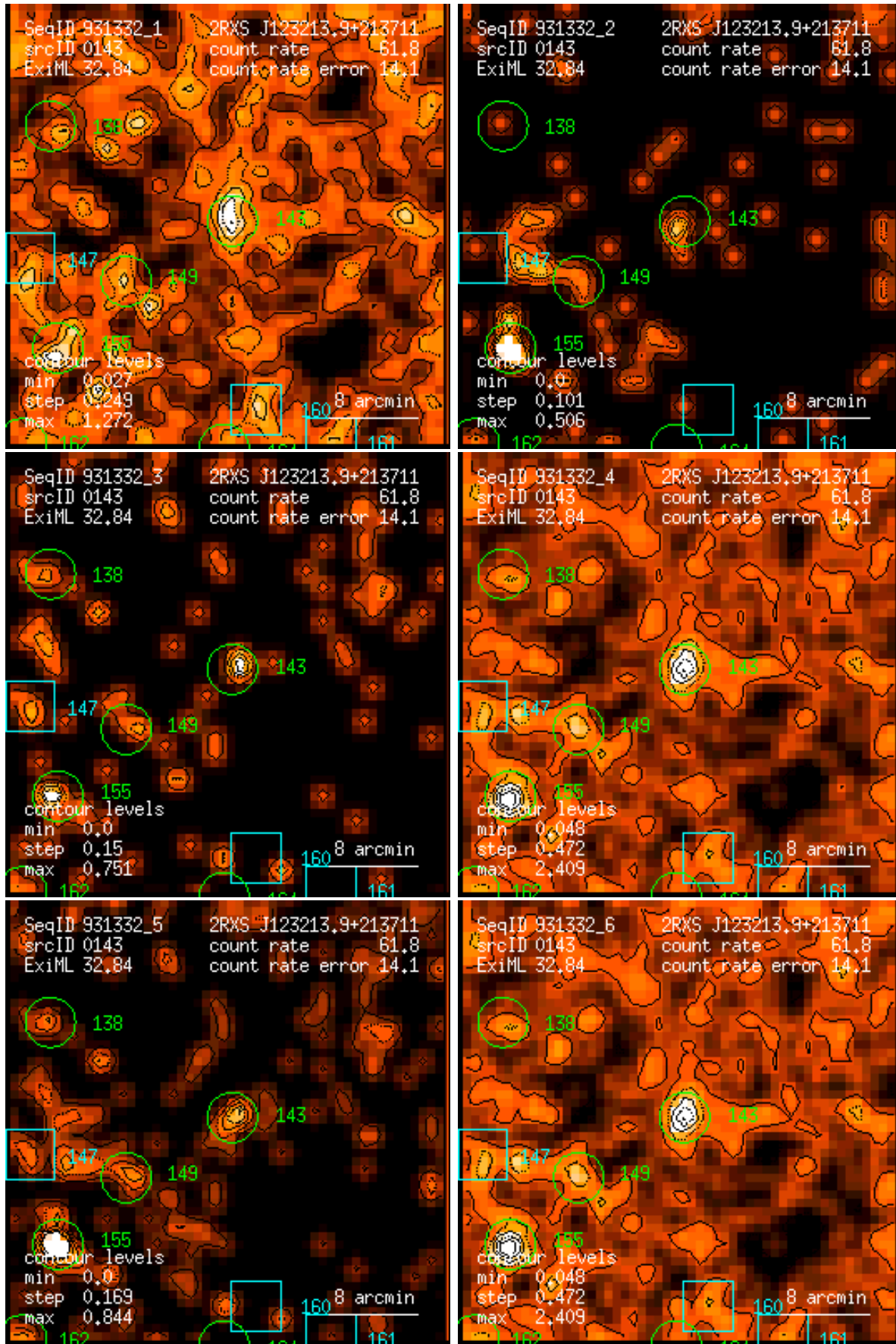
Figure 143: RASS 931332: detection 0143: band rate images, Gaussian filter: (1) PSPC channels 11 – 41, (2) 52 – 90, (3) 91 – 201, (4) 11 – 235, (5) 52 – 201, (6) 11 – 201. Broad band rates in counts/ks. Band rate contour levels in counts/ks/arcmin 2 .
