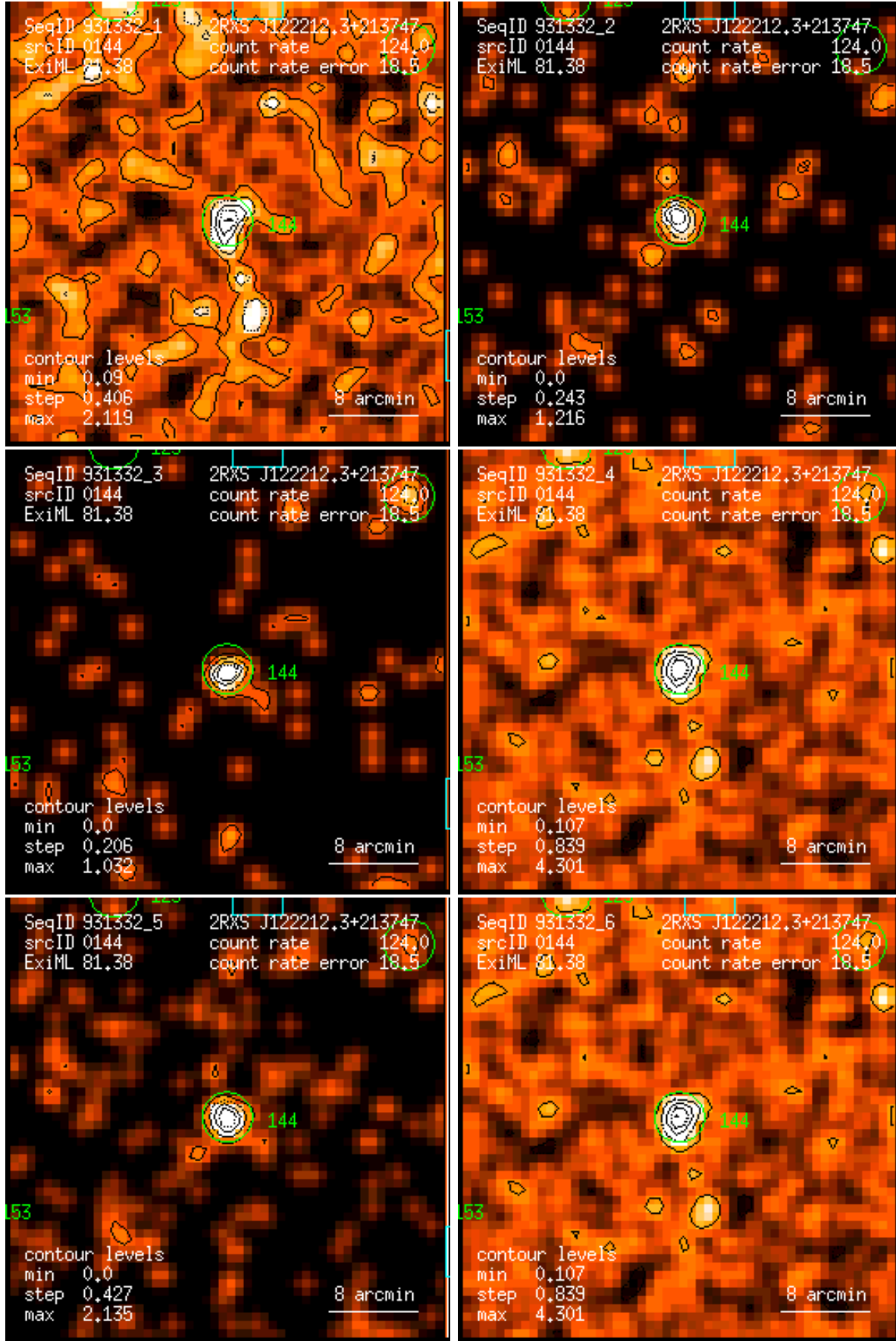
Figure 144: RASS 931332: detection 0144: band rate images, Gaussian filter: (1) PSPC channels 11 – 41, (2) 52 – 90, (3) 91 – 201, (4) 11 – 235, (5) 52 – 201, (6) 11 – 201. Broad band rates in counts/ks. Band rate contour levels in counts/ks/arcmin 2 .
