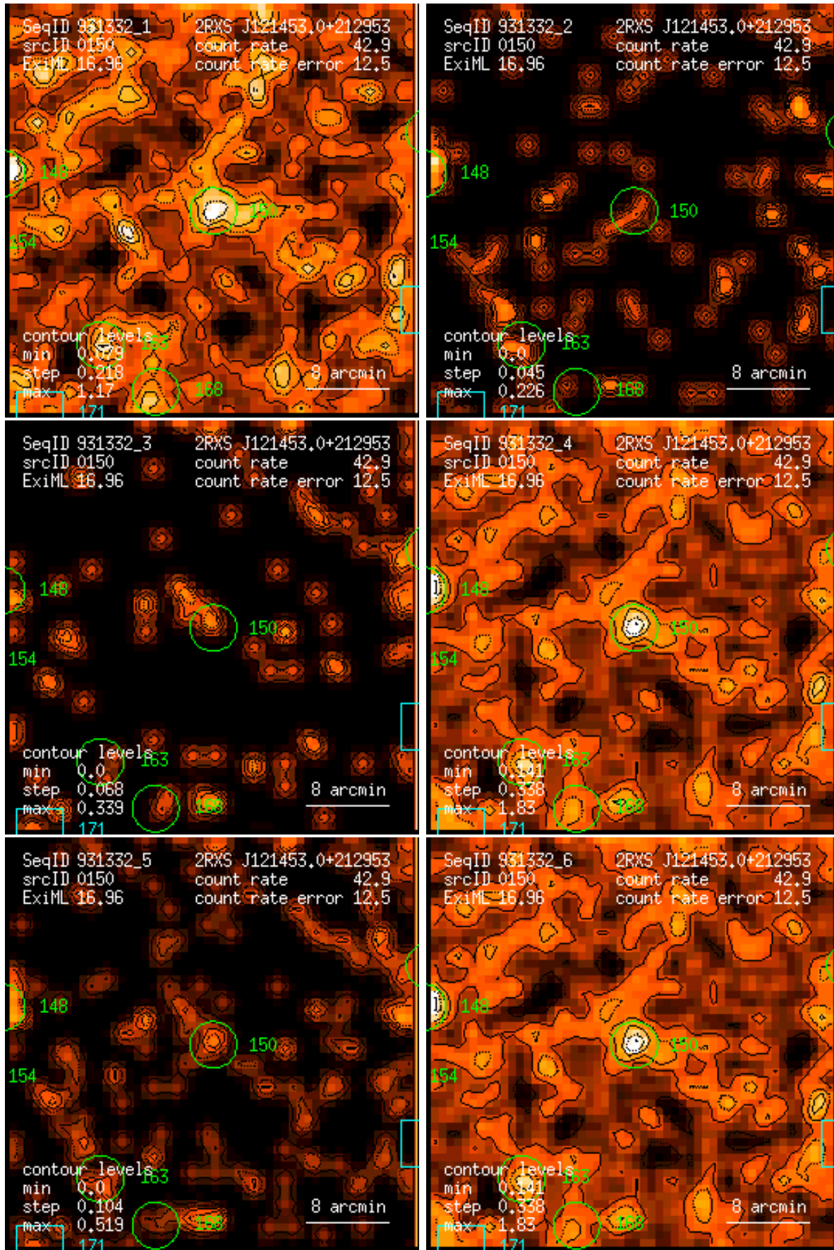
Figure 150: RASS 931332: detection 0150: band rate images, Gaussian filter: (1) PSPC channels 11 – 41, (2) 52 – 90, (3) 91 – 201, (4) 11 – 235, (5) 52 – 201, (6) 11 – 201. Broad band rates in counts/ks. Band rate contour levels in counts/ks/arcmin 2 .
