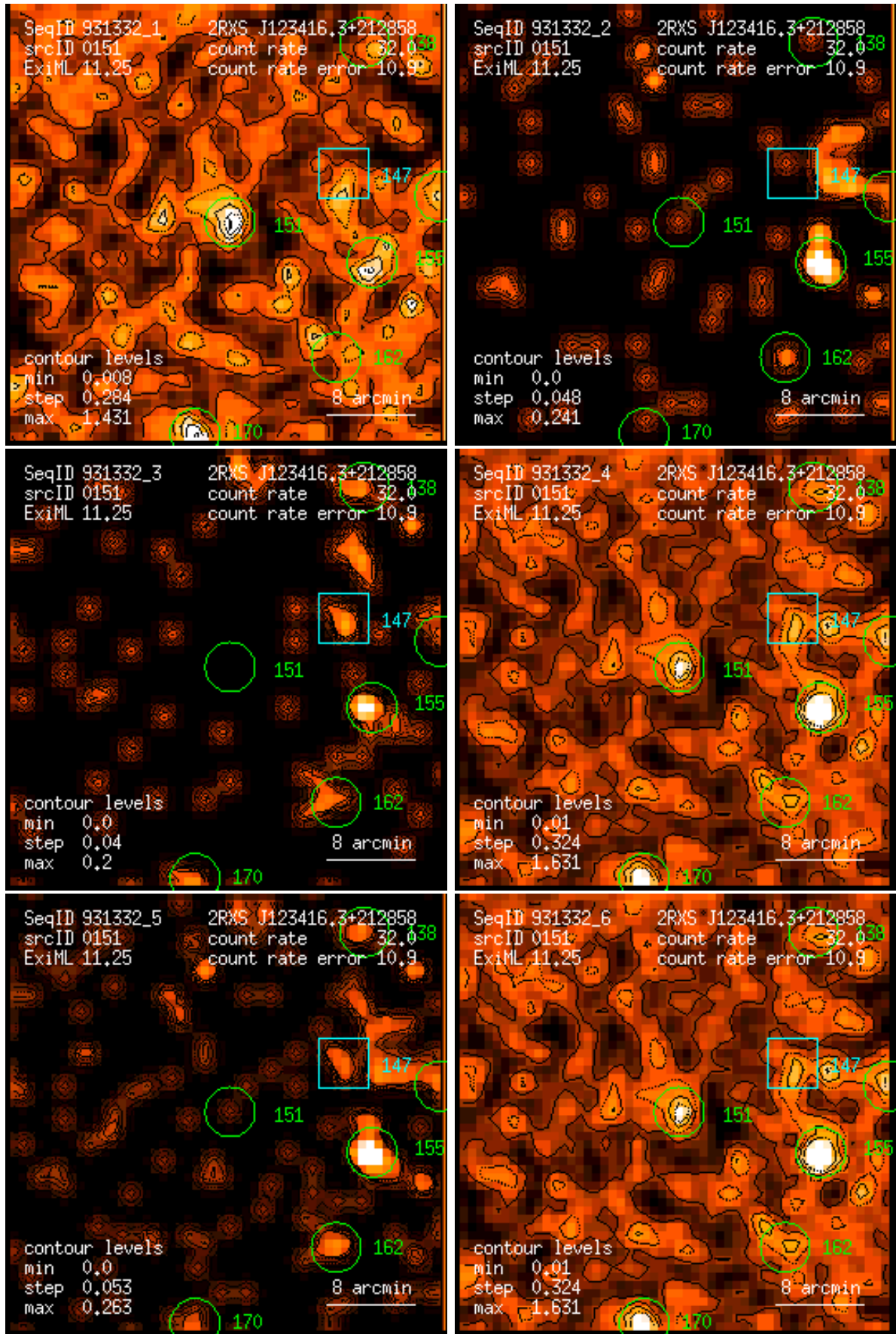
Figure 151: RASS 931332: detection 0151: band rate images, Gaussian filter: (1) PSPC channels 11 – 41, (2) 52 – 90, (3) 91 – 201, (4) 11 – 235, (5) 52 – 201, (6) 11 – 201. Broad band rates in counts/ks. Band rate contour levels in counts/ks/arcmin 2 .
