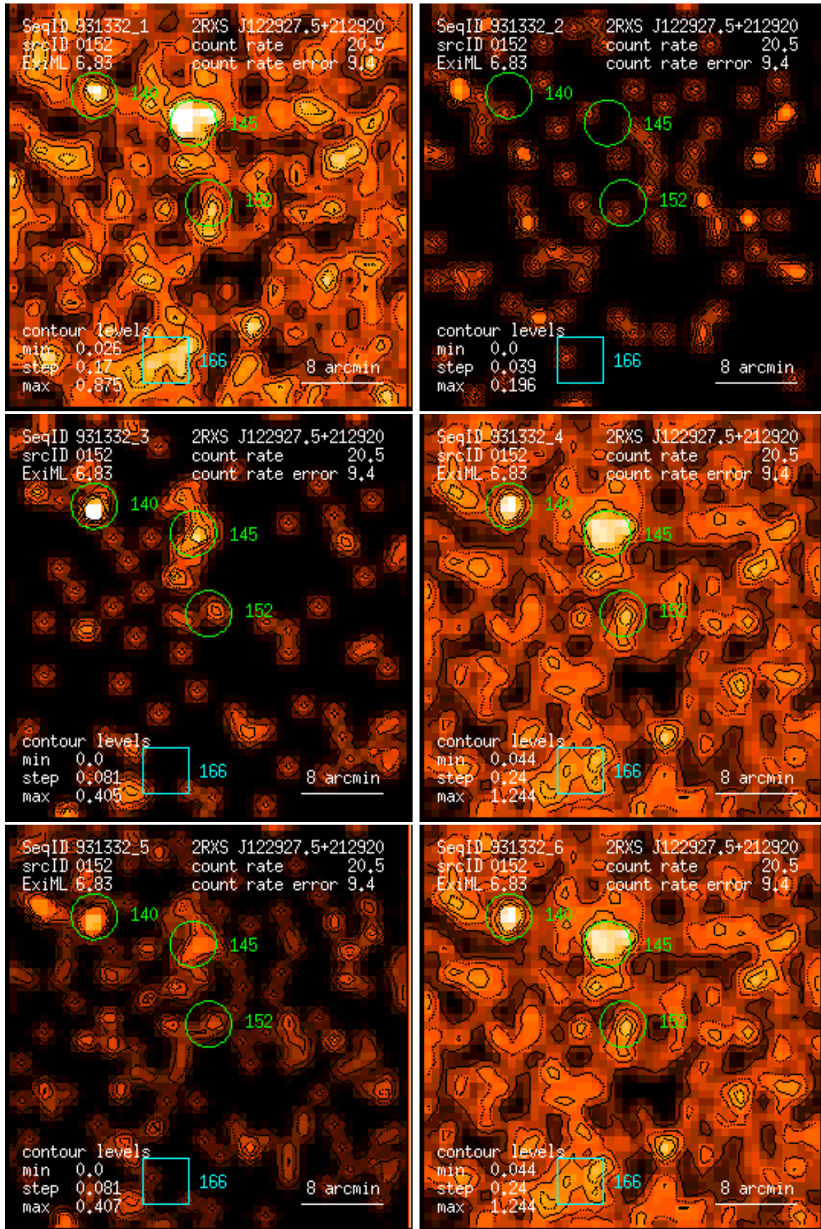
Figure 152: RASS 931332: detection 0152: band rate images, Gaussian filter: (1) PSPC channels 11 – 41, (2) 52 – 90, (3) 91 – 201, (4) 11 – 235, (5) 52 – 201, (6) 11 – 201. Broad band rates in counts/ks. Band rate contour levels in counts/ks/arcmin 2 .
