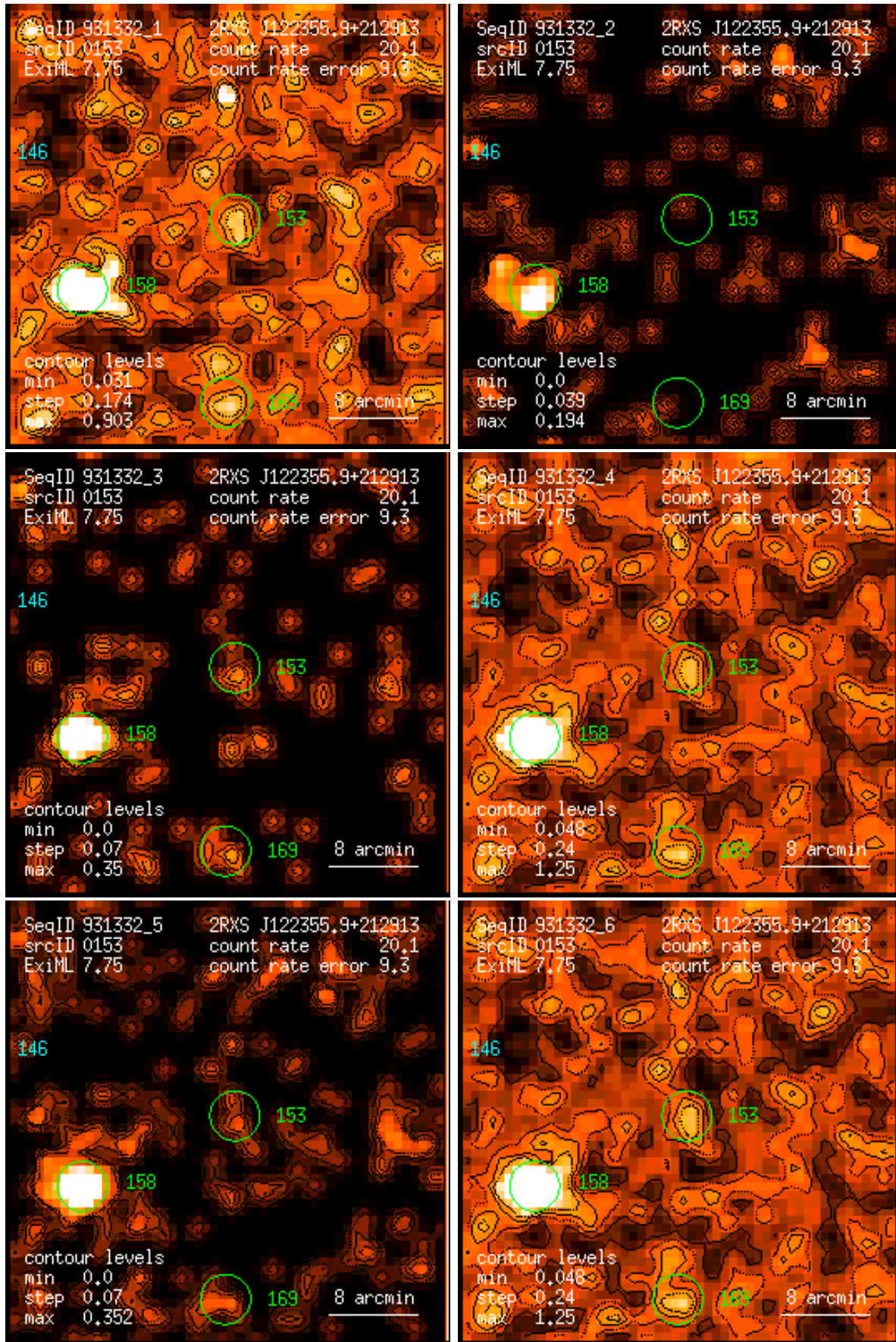
Figure 153: RASS 931332: detection 0153: band rate images, Gaussian filter: (1) PSPC channels 11 – 41, (2) 52 – 90, (3) 91 – 201, (4) 11 – 235, (5) 52 – 201, (6) 11 – 201. Broad band rates in counts/ks. Band rate contour levels in counts/ks/arcmin 2 .
