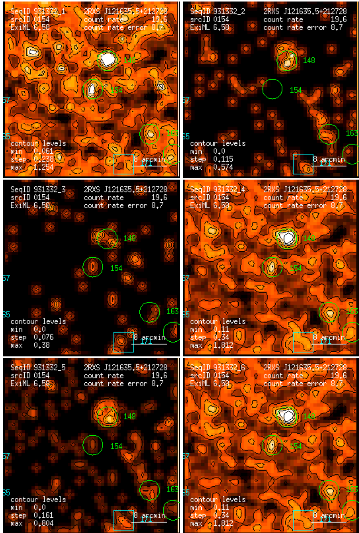
Figure 154: RASS 931332: detection 0154: band rate images, Gaussian filter: (1) PSPC channels 11 – 41, (2) 52 – 90, (3) 91 – 201, (4) 11 – 235, (5) 52 – 201, (6) 11 – 201. Broad band rates in counts/ks. Band rate contour levels in counts/ks/arcmin 2 .
