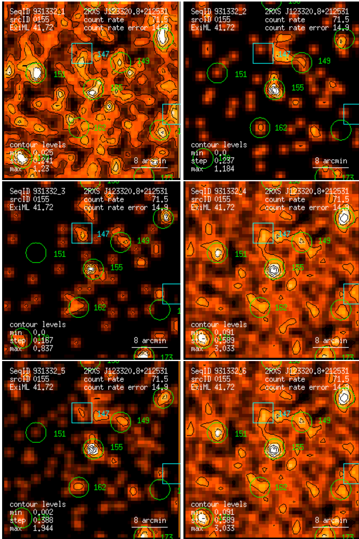
Figure 155: RASS 931332: detection 0155: band rate images, Gaussian filter: (1) PSPC channels 11 – 41, (2) 52 – 90, (3) 91 – 201, (4) 11 – 235, (5) 52 – 201, (6) 11 – 201. Broad band rates in counts/ks. Band rate contour levels in counts/ks/arcmin 2 .
