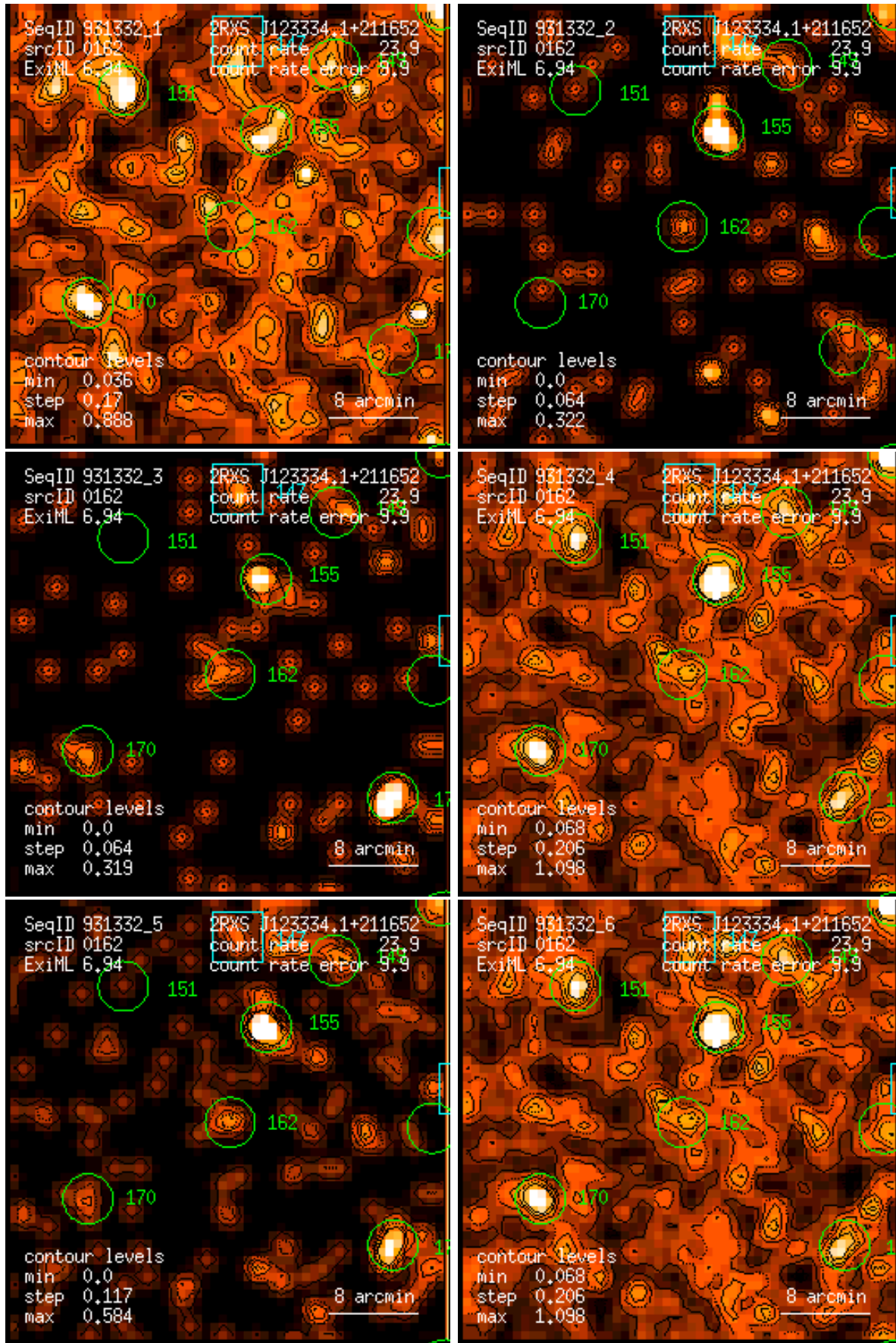
Figure 162: RASS 931332: detection 0162: band rate images, Gaussian filter: (1) PSPC channels 11 – 41, (2) 52 – 90, (3) 91 – 201, (4) 11 – 235, (5) 52 – 201, (6) 11 – 201. Broad band rates in counts/ks. Band rate contour levels in counts/ks/arcmin 2 .
