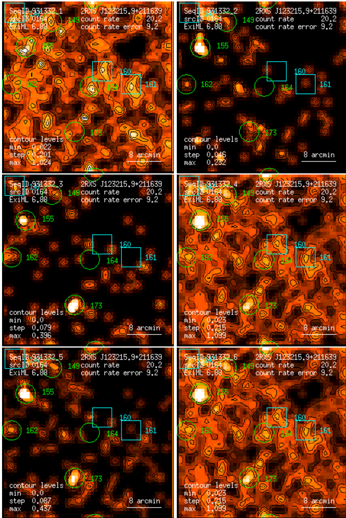
Figure 164: RASS 931332: detection 0164: band rate images, Gaussian filter: (1) PSPC channels 11 – 41, (2) 52 – 90, (3) 91 – 201, (4) 11 – 235, (5) 52 – 201, (6) 11 – 201. Broad band rates in counts/ks. Band rate contour levels in counts/ks/arcmin 2 .
