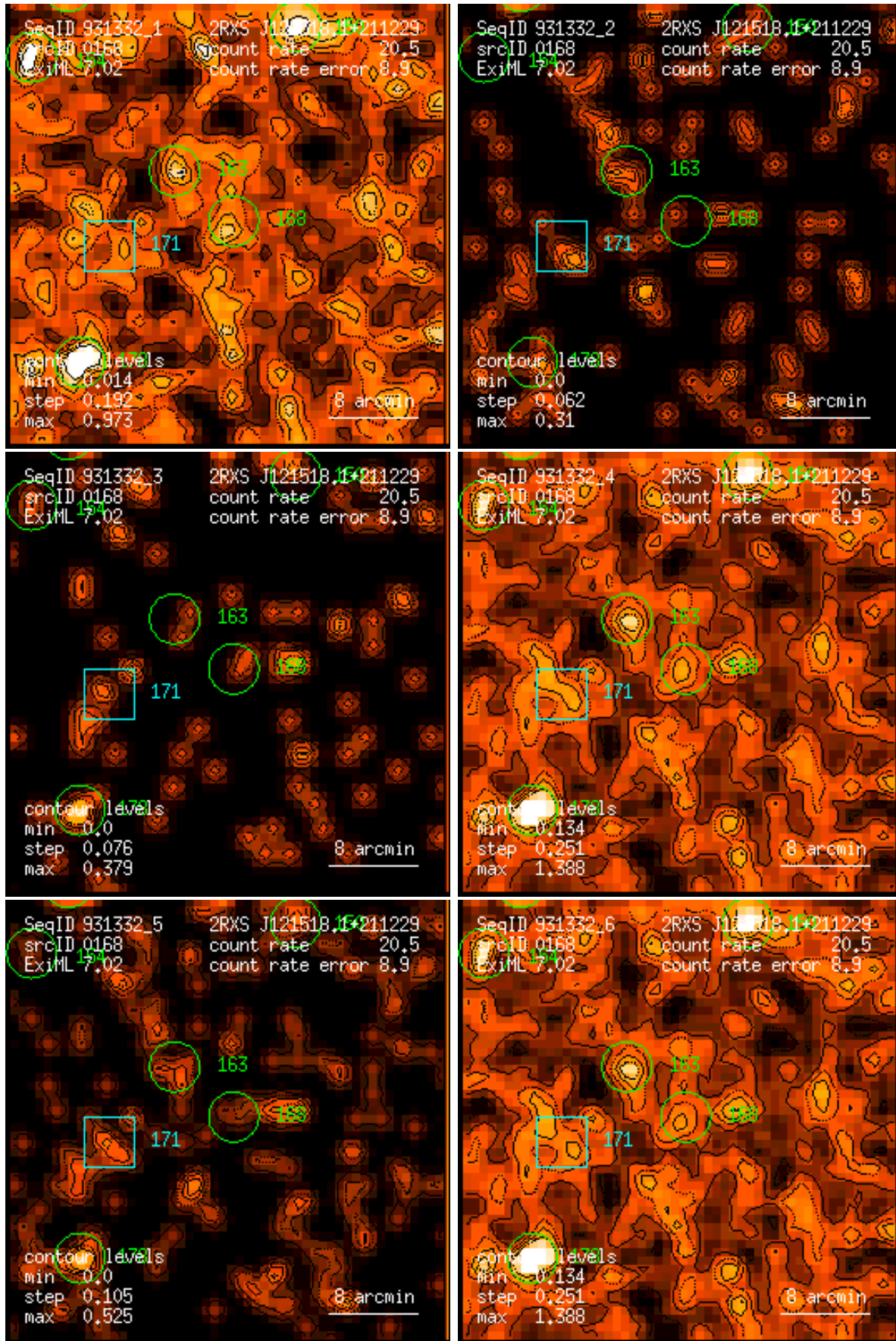
Figure 168: RASS 931332: detection 0168: band rate images, Gaussian filter: (1) PSPC channels 11 – 41, (2) 52 – 90, (3) 91 – 201, (4) 11 – 235, (5) 52 – 201, (6) 11 – 201. Broad band rates in counts/ks. Band rate contour levels in counts/ks/arcmin 2 .
